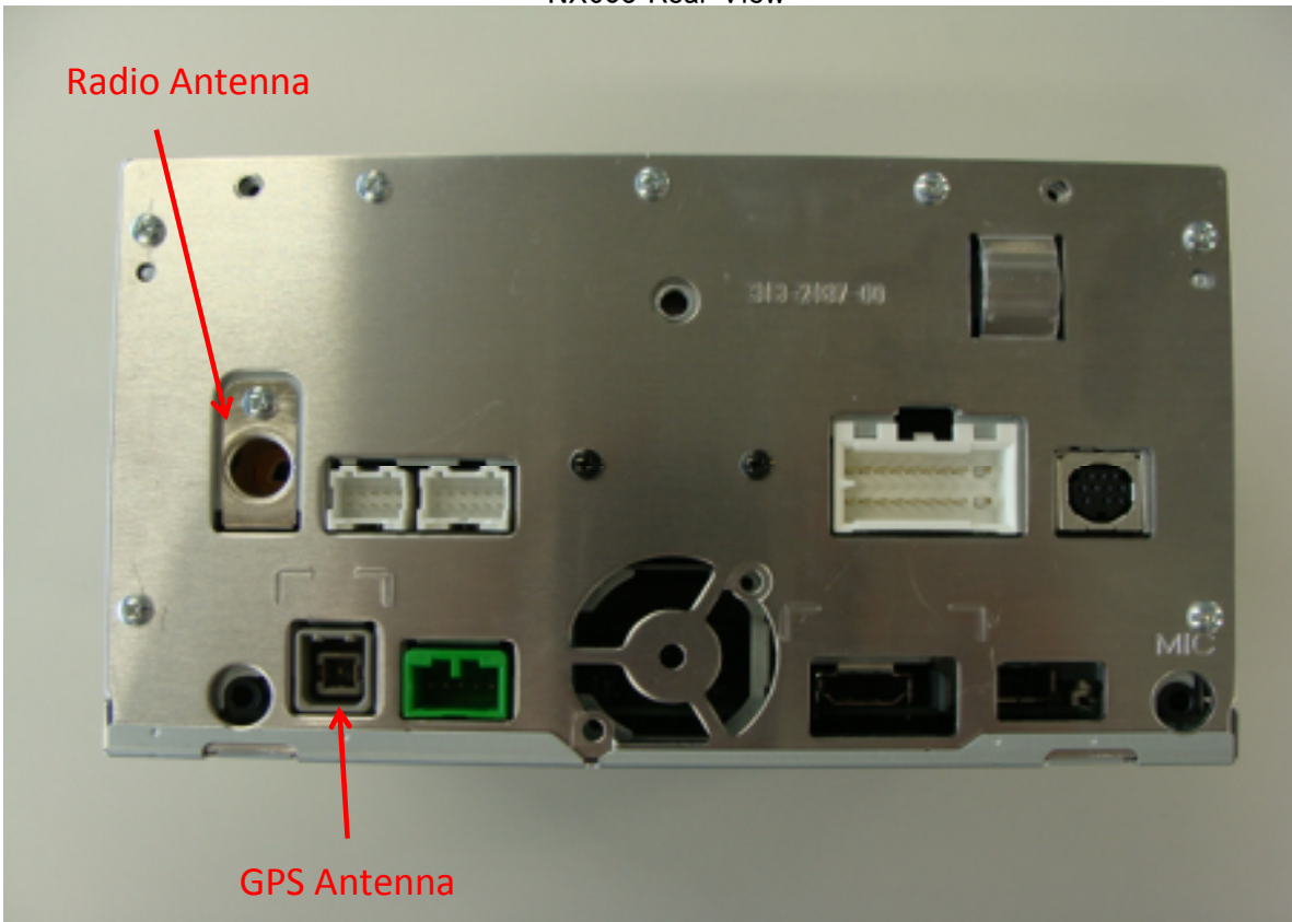
NX603 Rear View
