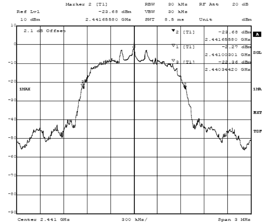
Title: 20dB Bandwidth Comment A: CH M: 2441 MHz; 20dB bandwidth (kHz):1311.6
