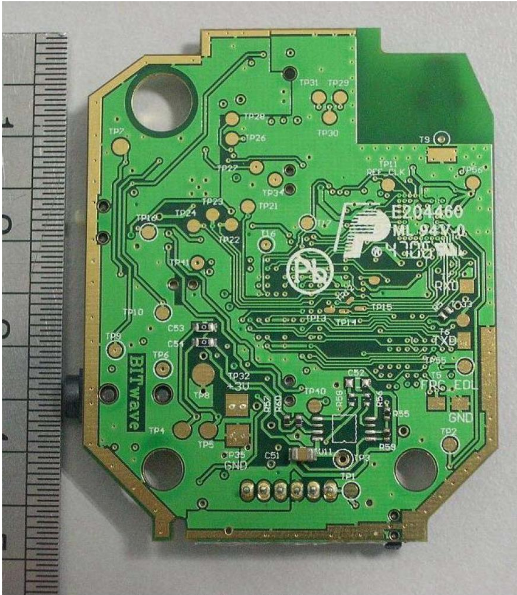
Main-Board - PCB Trace Side
