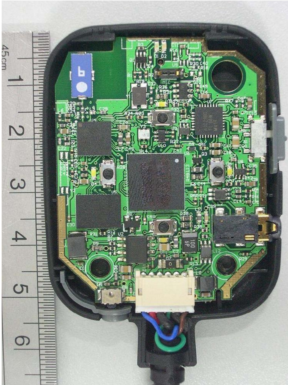
EUT Internal View
