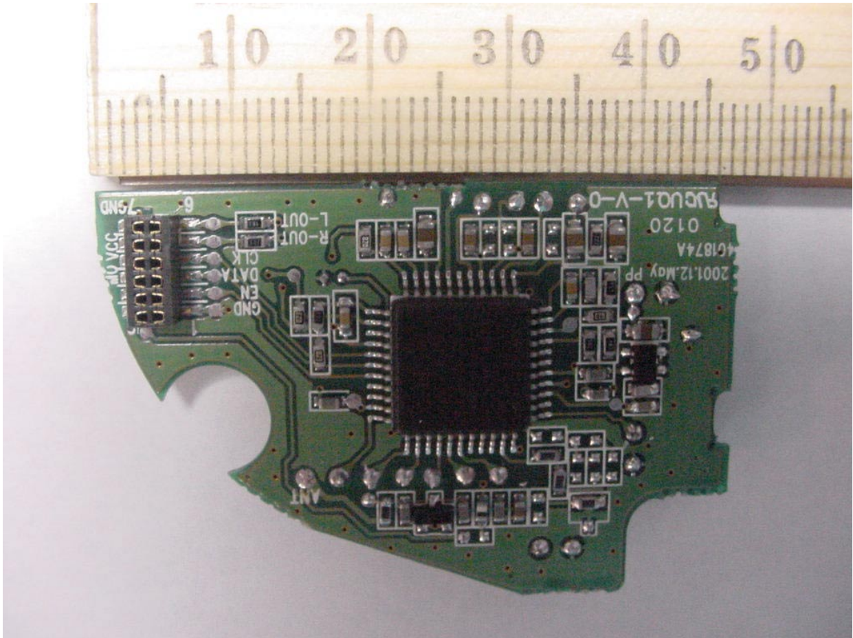
Sub-PCB Front
