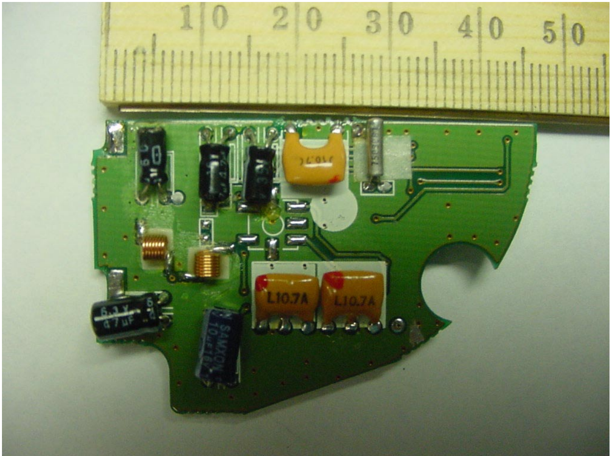
Sub-PC Back
