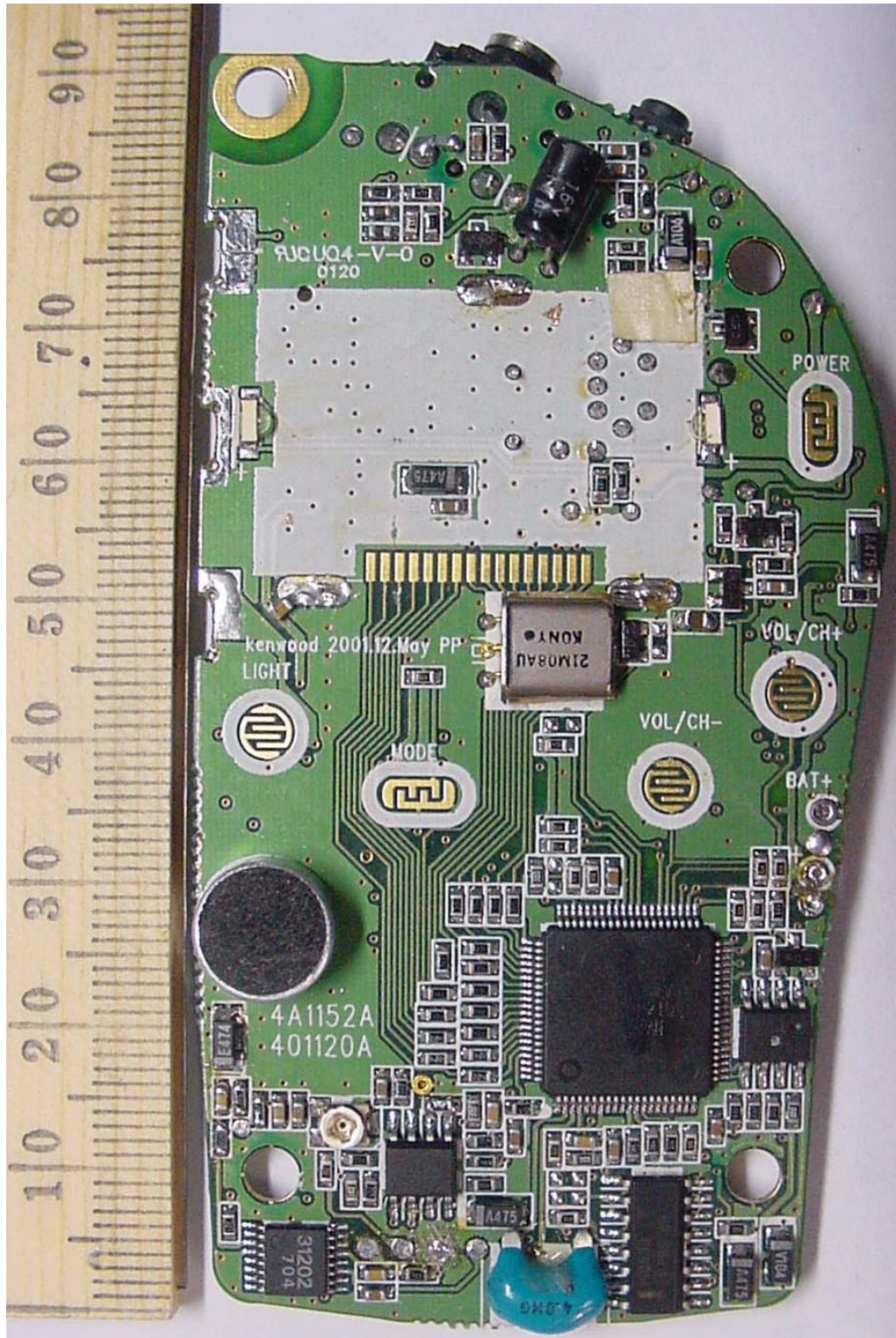
Front of Main PCB with LCD removed
