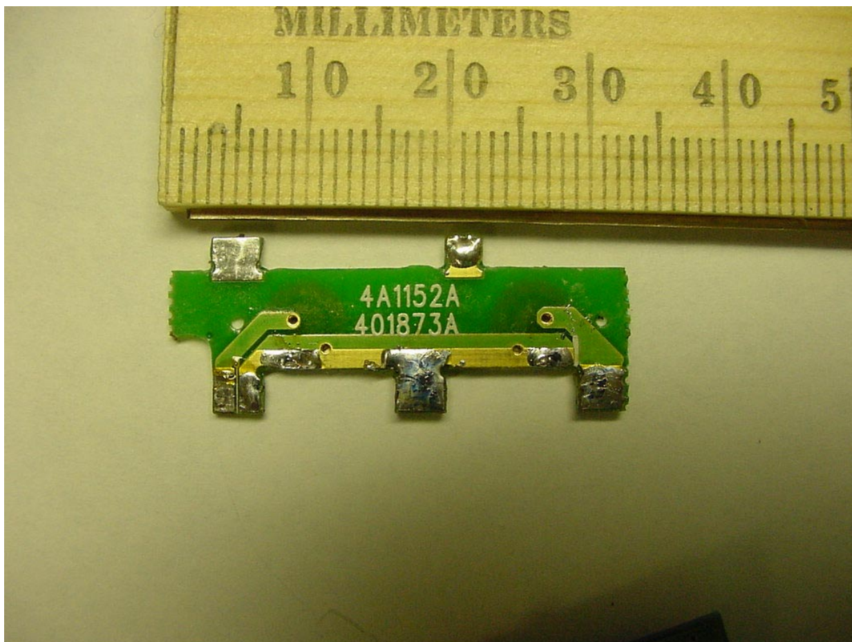
Inside of switch PCB
