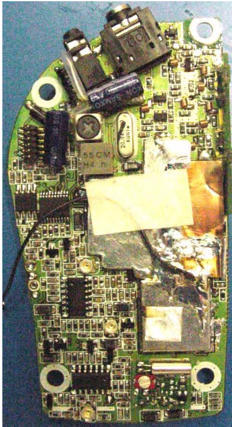
Back of Main PCB with shields
