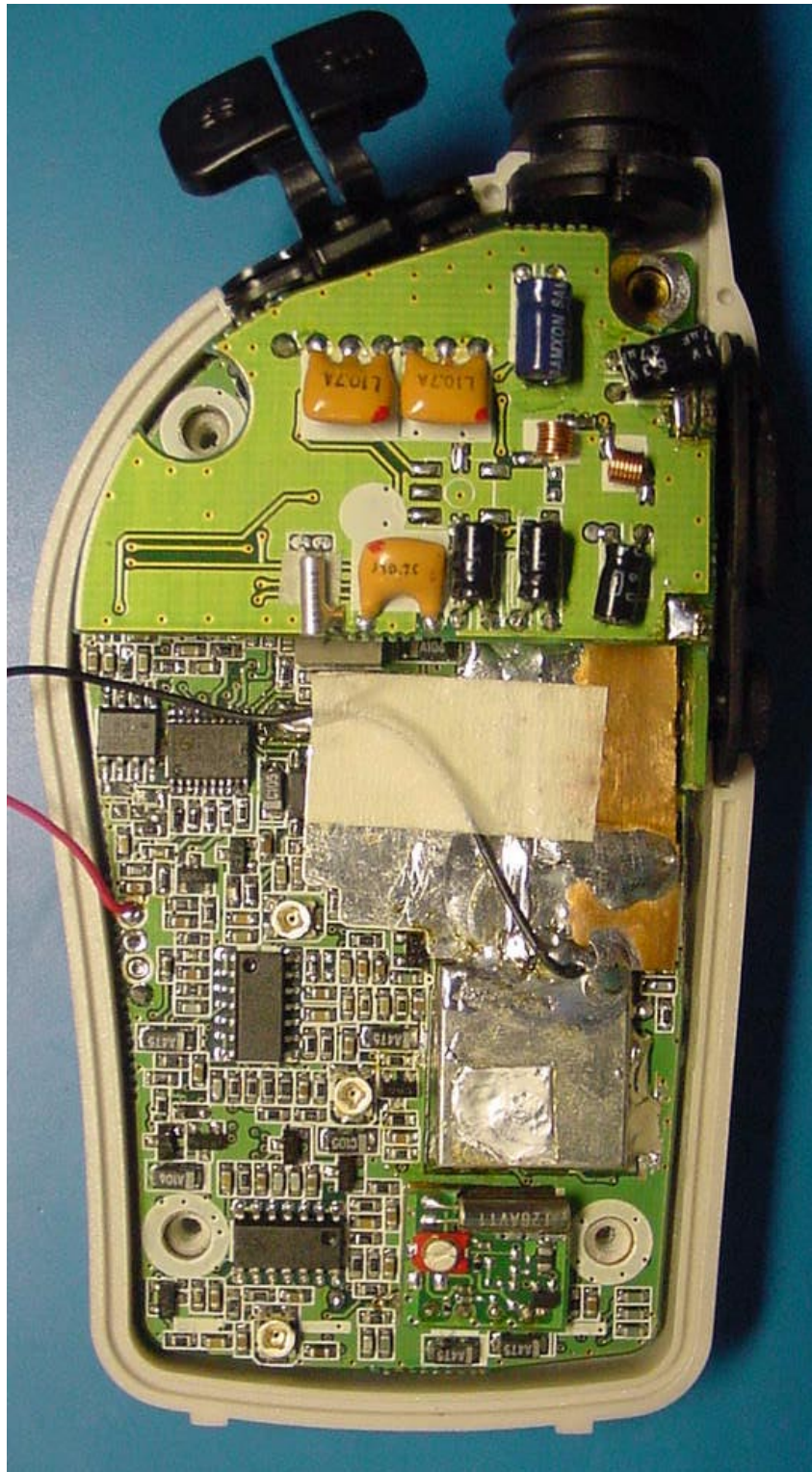
Back of Main PCB in Case
