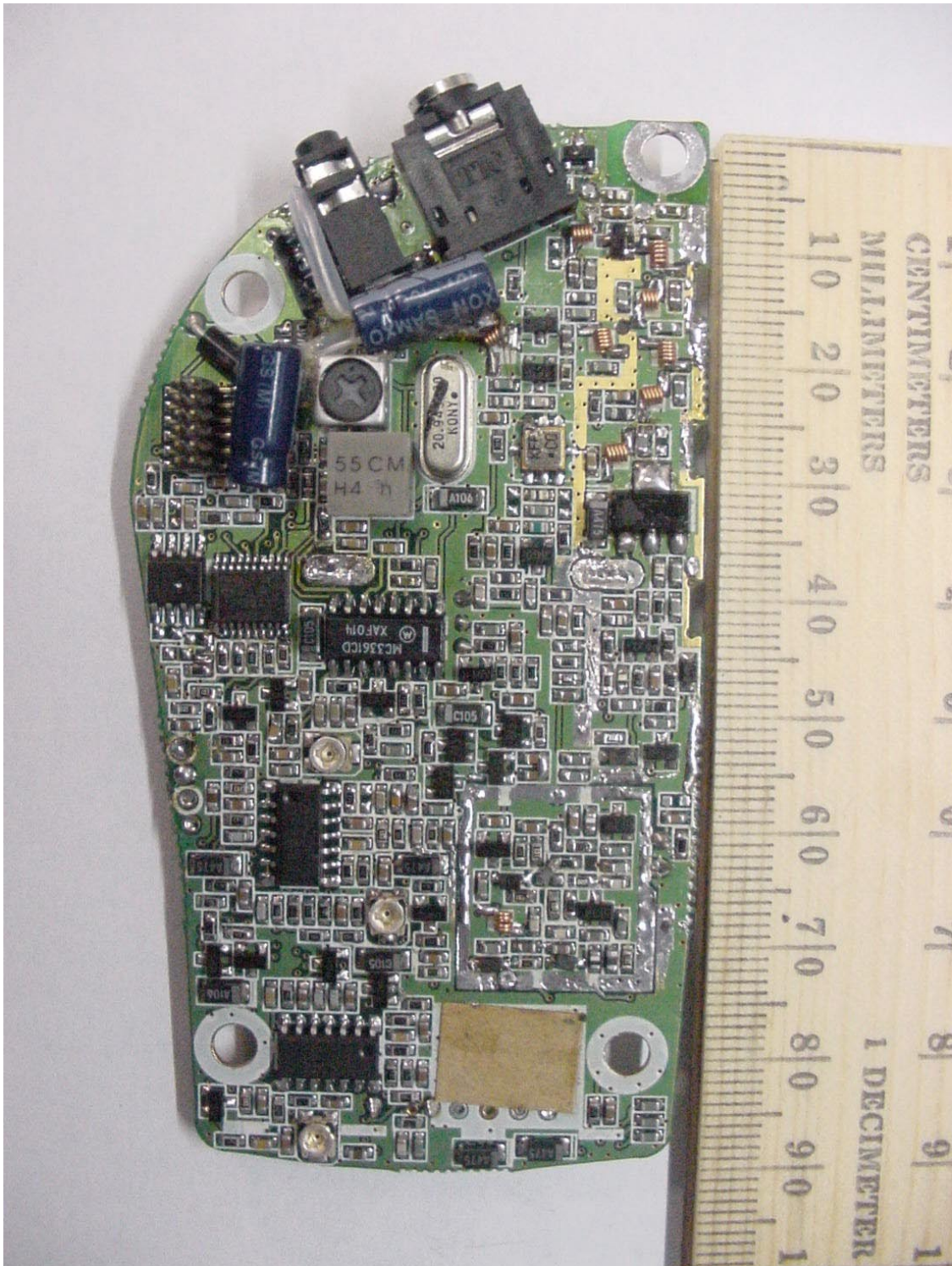
Back of Main PCB Shields removed
