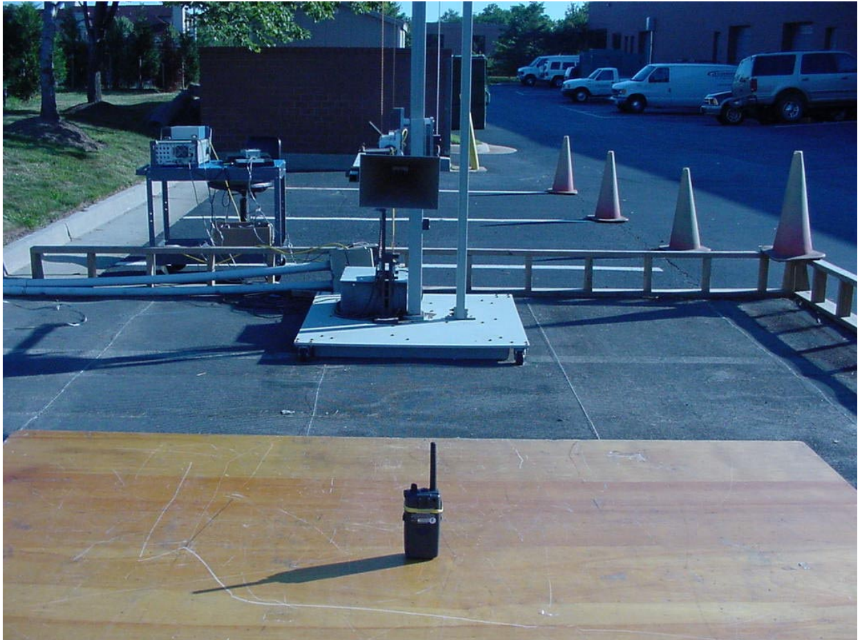
PHOTOGRAPH 1: RADIATED TEST CONFIGURATION (REAR VIEW)
