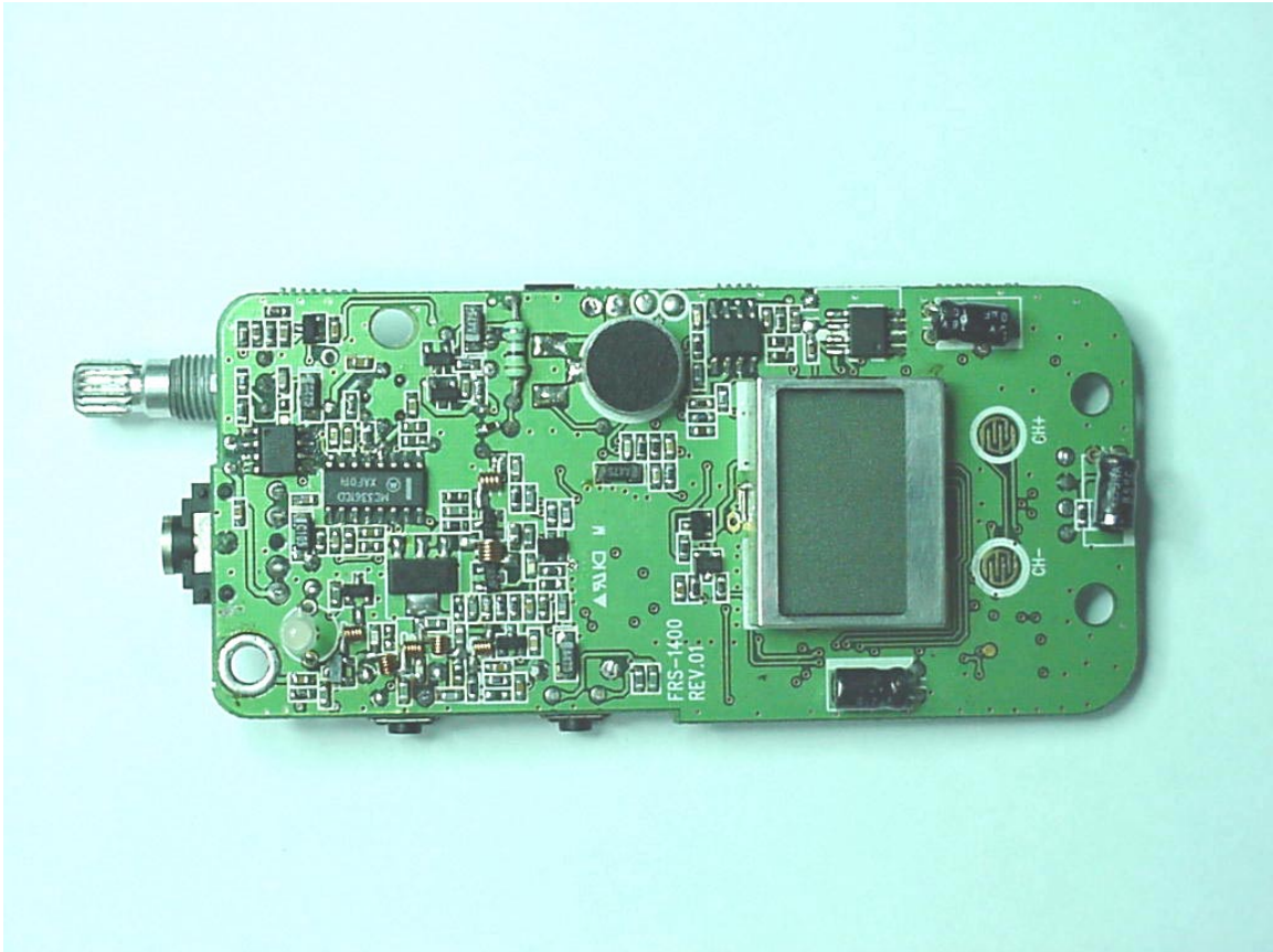
PHOTOGRAPH 8: FRONT VIEW OF PCB WITH SHIELDS REMOVED
