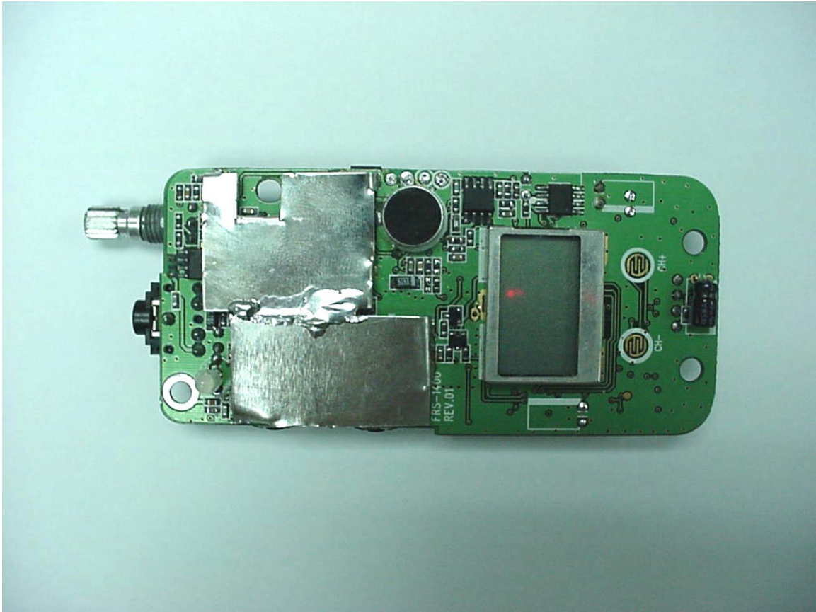
PHOTOGRAPH 10: FRONT VIEW OF PCB WITH SHIELDS
