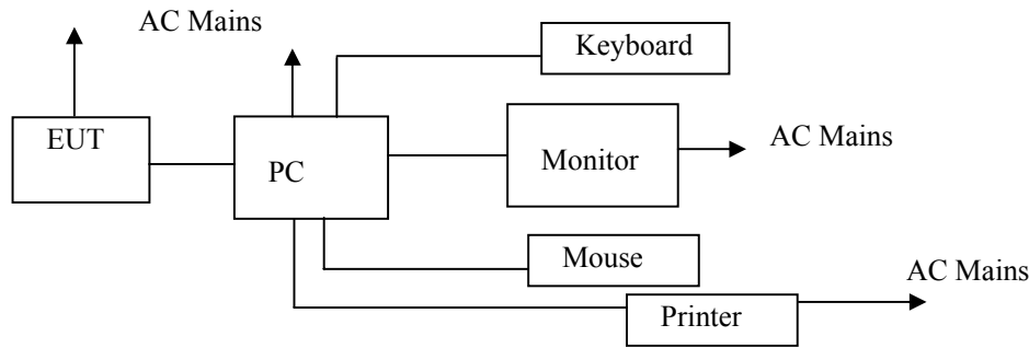
Fig. 2-1 Configuration of Tested System
