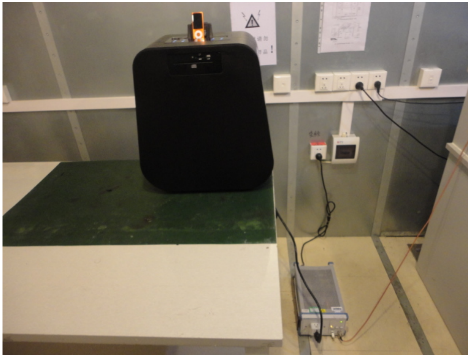
Conducted Emission Setup:
