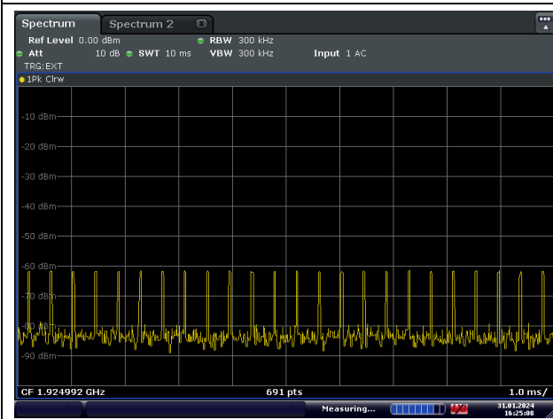
35 \mu s Pulses
