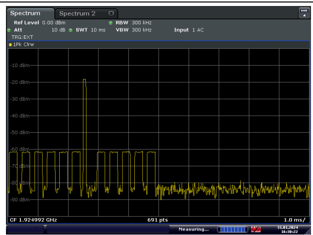
Access Criteria Check, Functional Test, After
