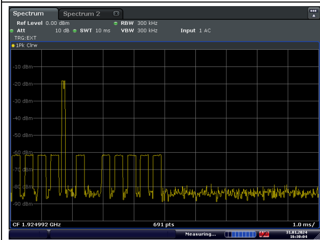
Access Criteria Check, Functional Test, Before
