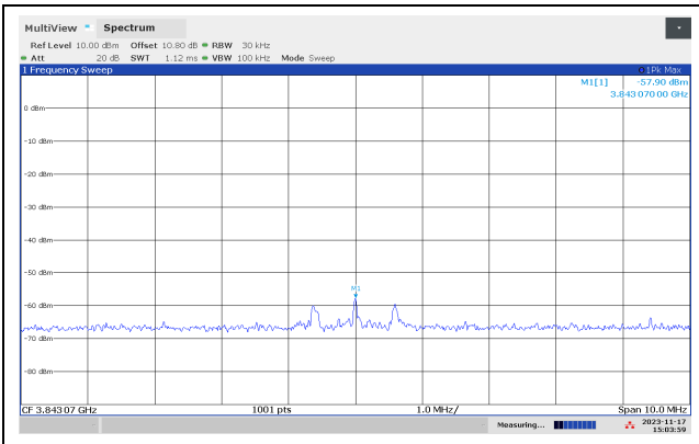
Out-of-Band Emissions 3843 MHz, Lower Channel
