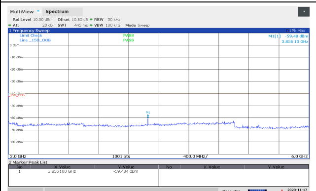
Out-of-Band Emissions, Upper Channel
