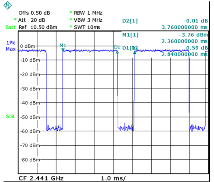
Middle Channel
