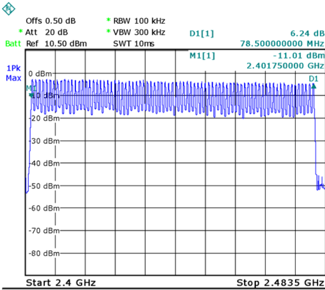
Modulation: GFSK
