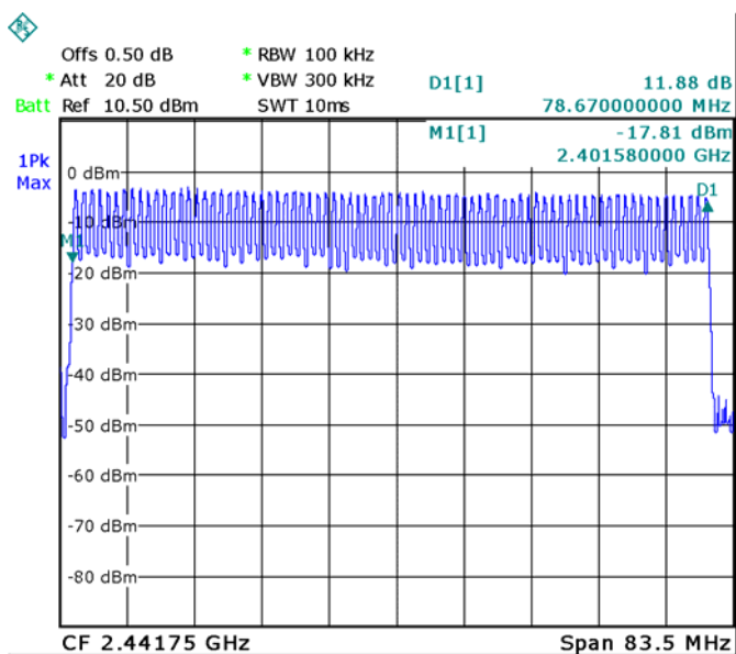
Modulation: GFSK
