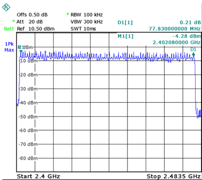
Modulation: 8DPSK
