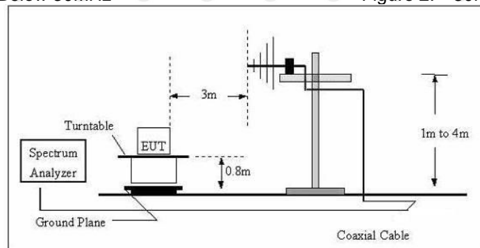
Figure 3. Above 1GHz
