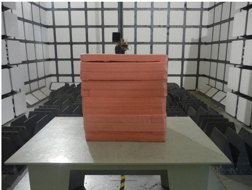
Transmitting Radiated Emissions (Above 1 GHz)
