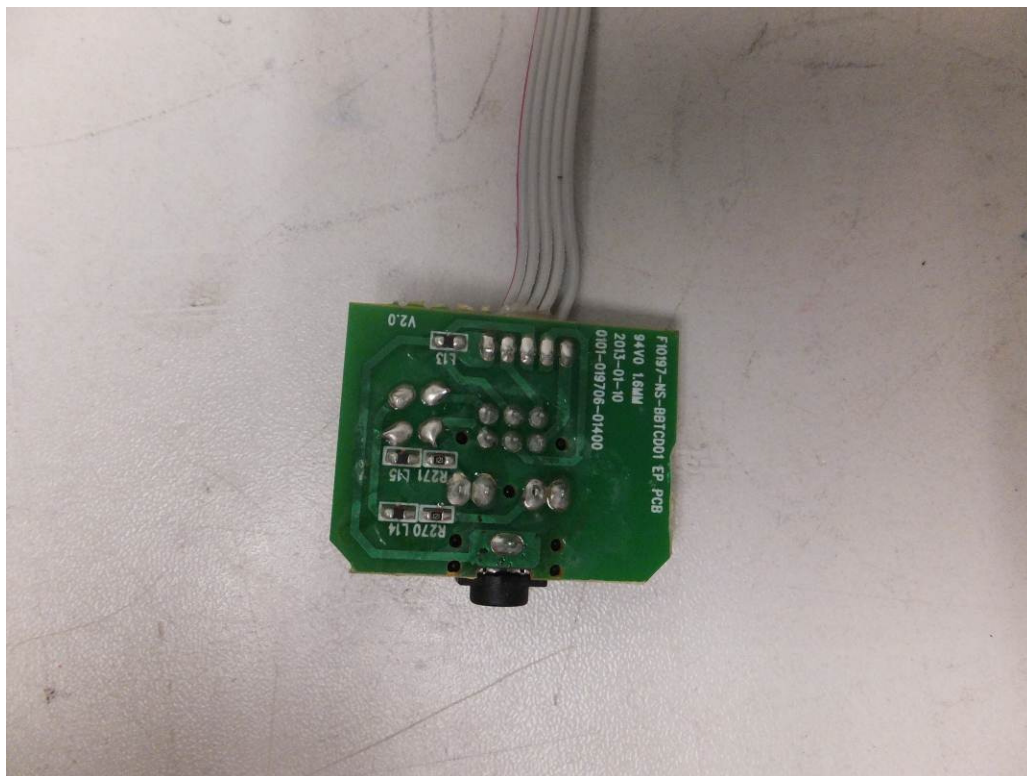
Fig. 10: Internal view
