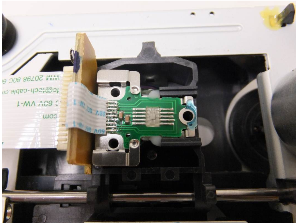
Fig. 25: Internal view
