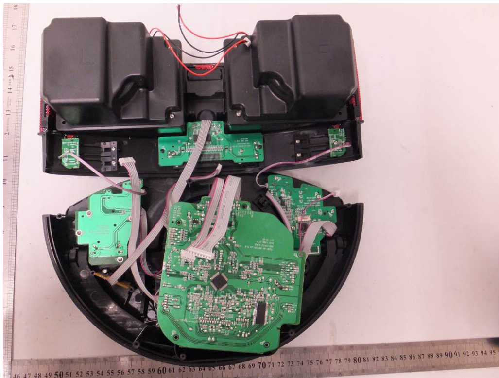
Fig. 2: Internal view
