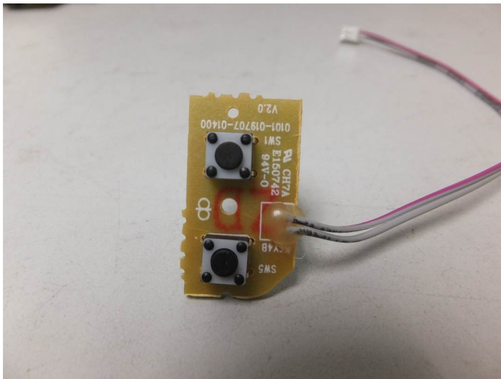
Fig. 14: Internal view
