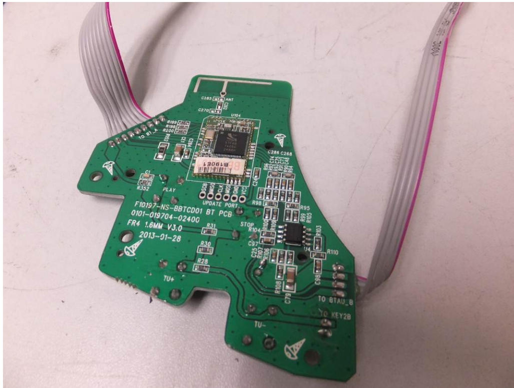
Fig. 19: Internal view
