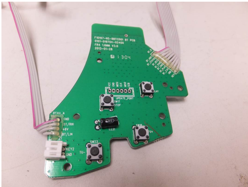
Fig. 18: Internal view
