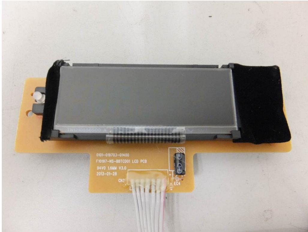
Fig. 9: Internal view
