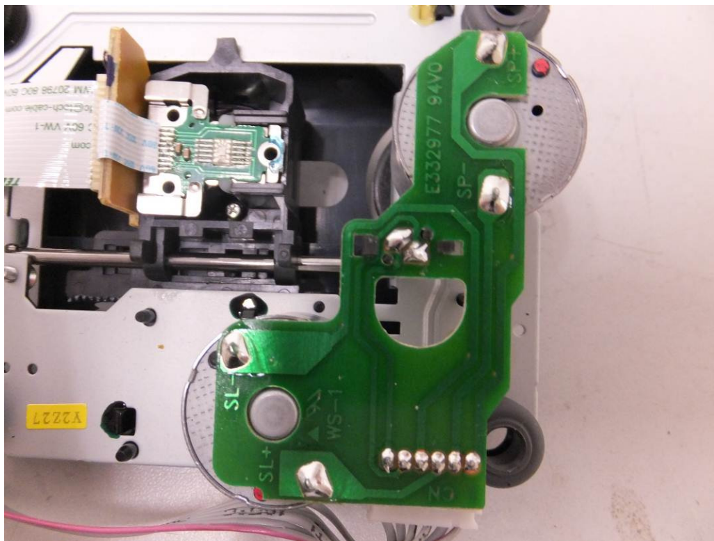
Fig. 24: Internal view
