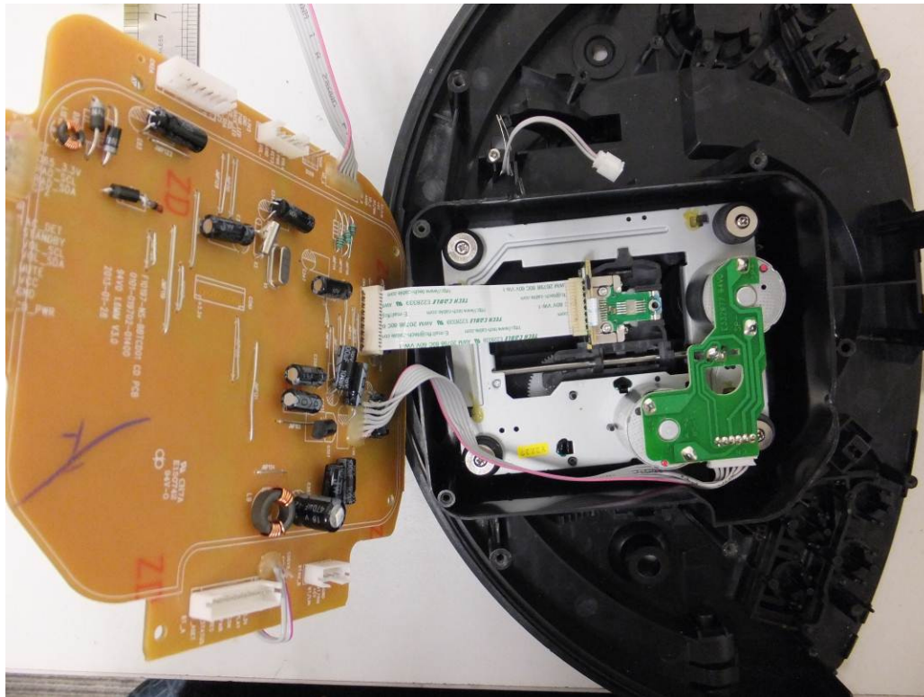
Fig. 23: Internal view
