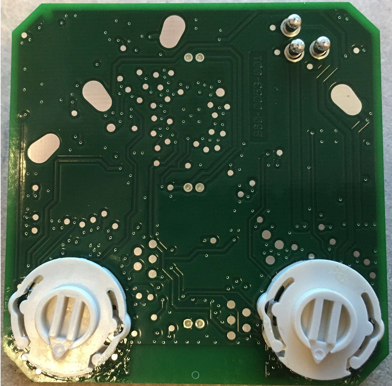
PCB Bottom:
