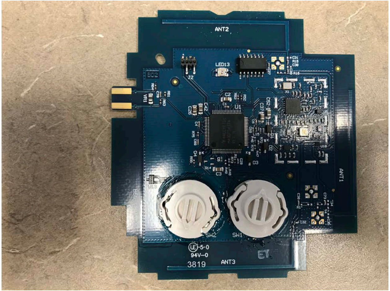
Internal – Front
