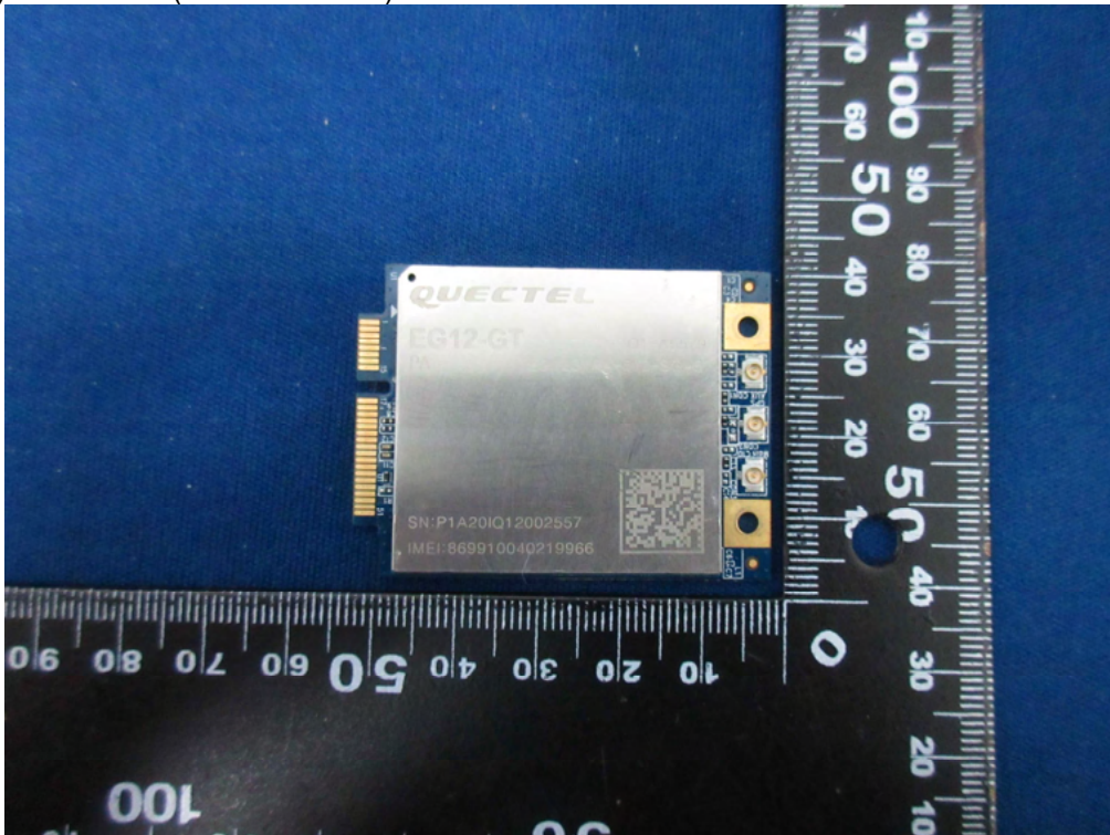
(18) EUT Photo (WWAN Module)
