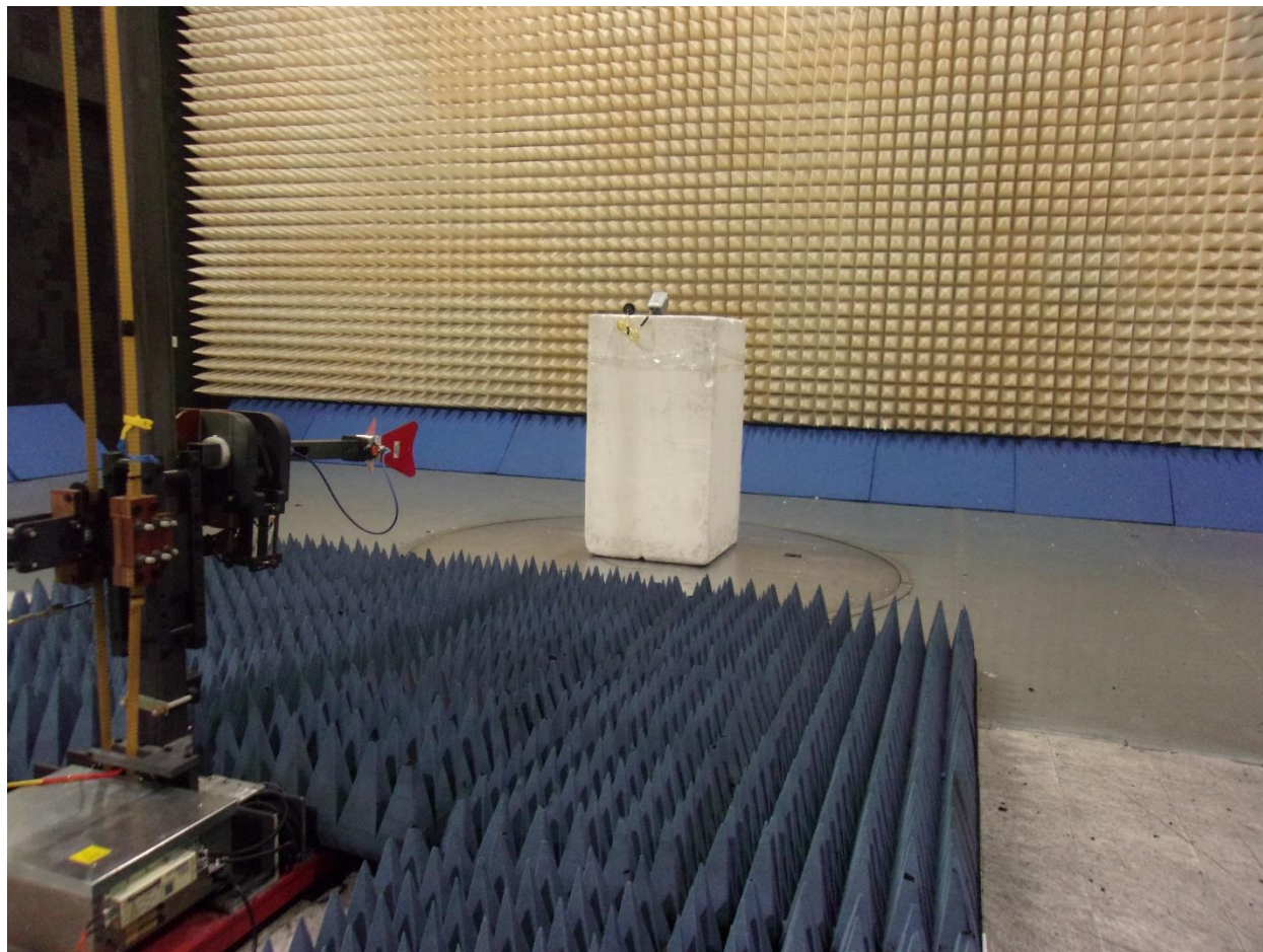
Radiated Spurious Emissions, 1 – 18GHz
