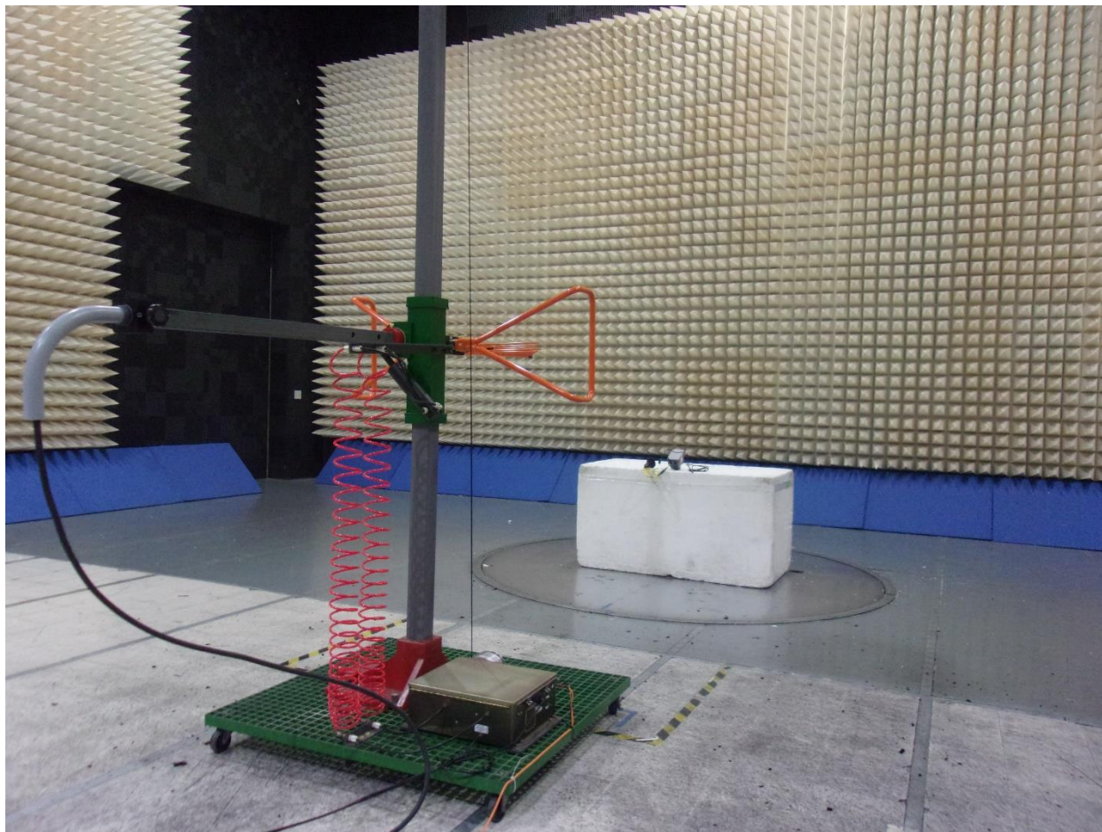
Unintentional and Spurious Emissions, 30MHz – 1GHz
