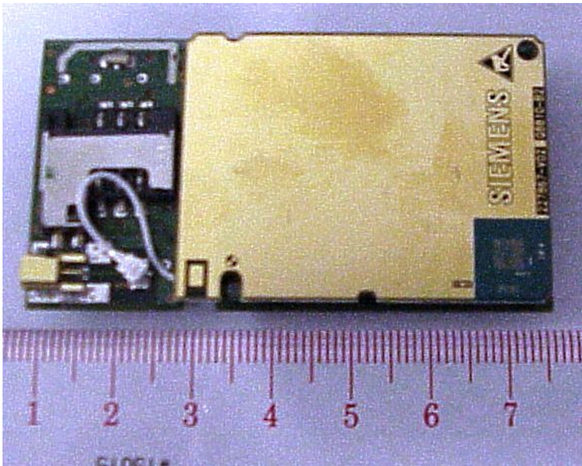
MTSMC-G with TC63 component side
