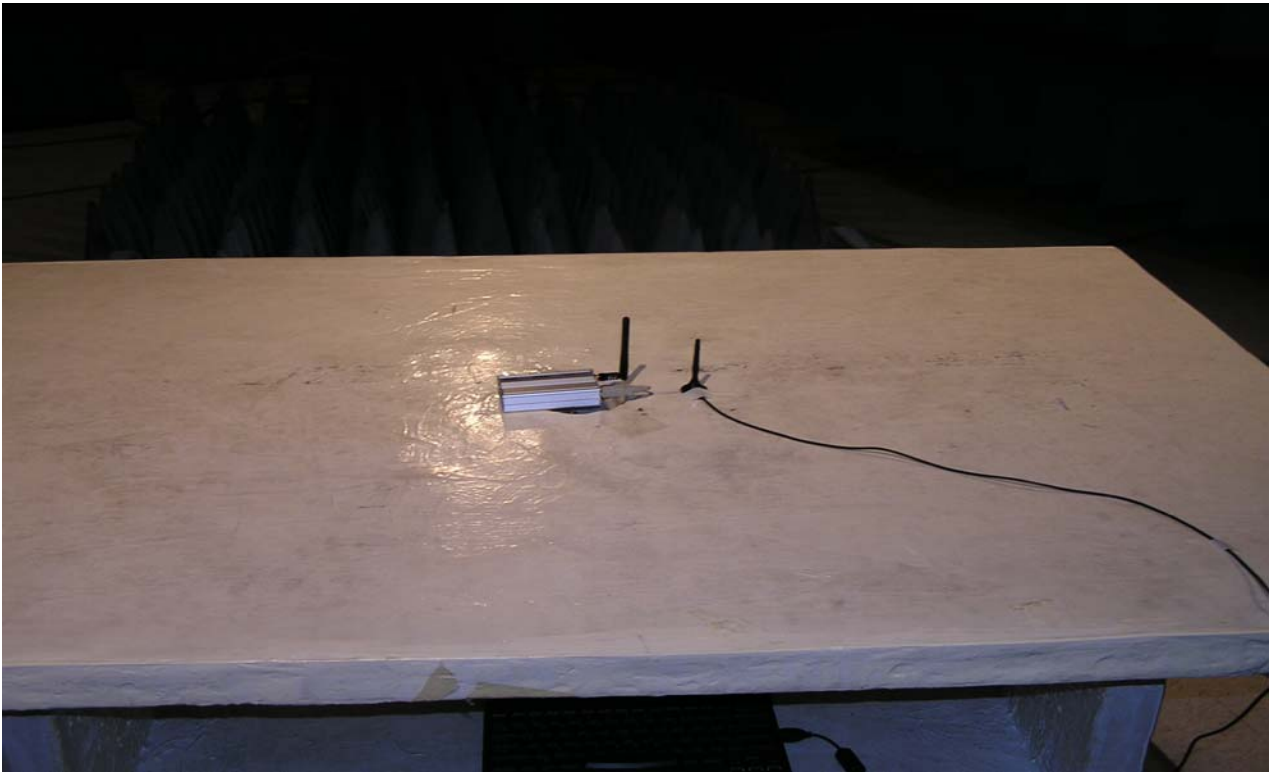
RADIATED EMISSIONS ABOVE 1GHz
