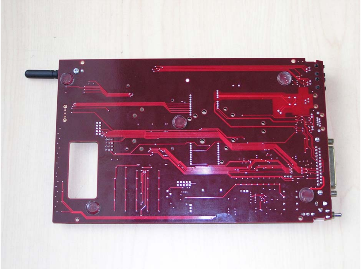
MTMMC-C in test fixture – Bottom view
