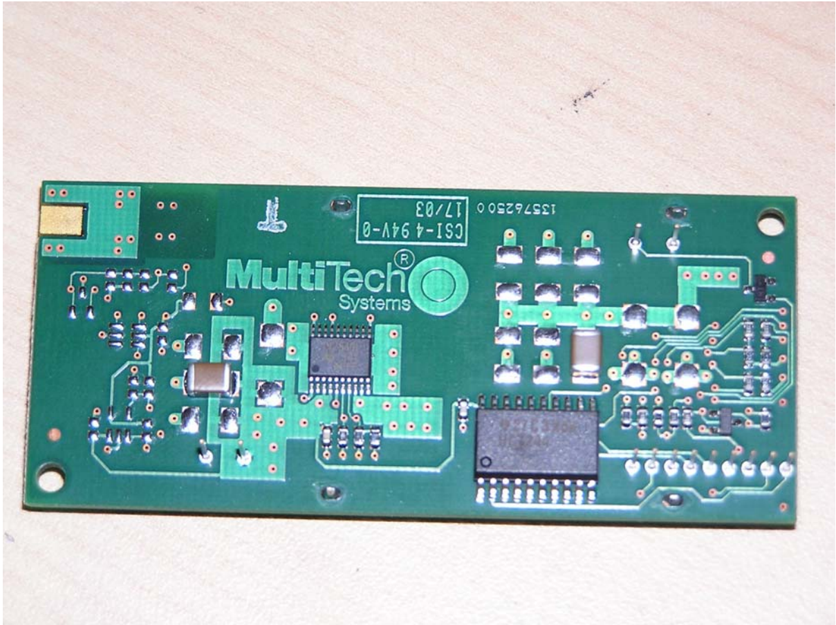
MTSMC-C – PCB Bottom view
