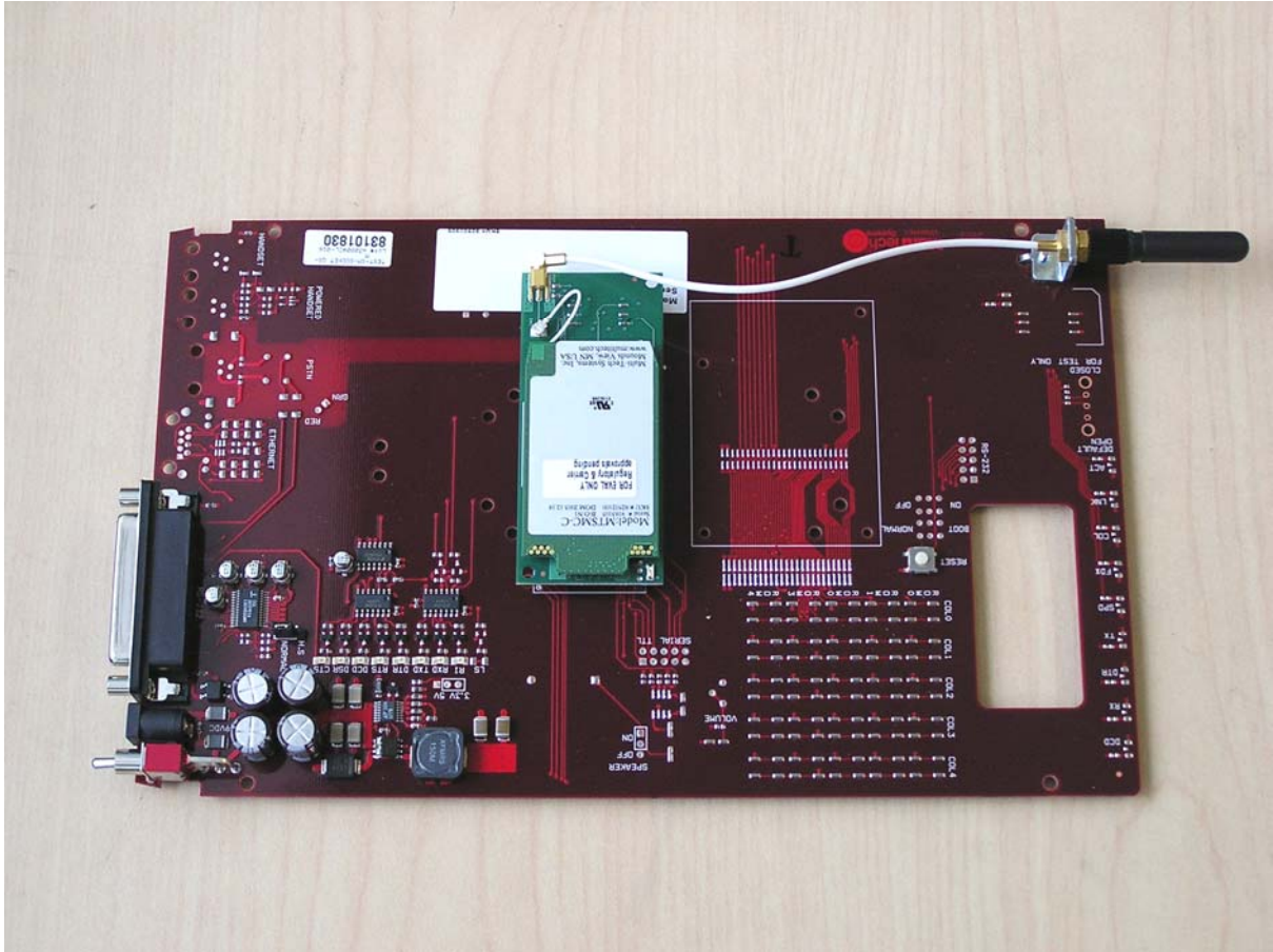
MTSMC-C in test fixture – Top view
