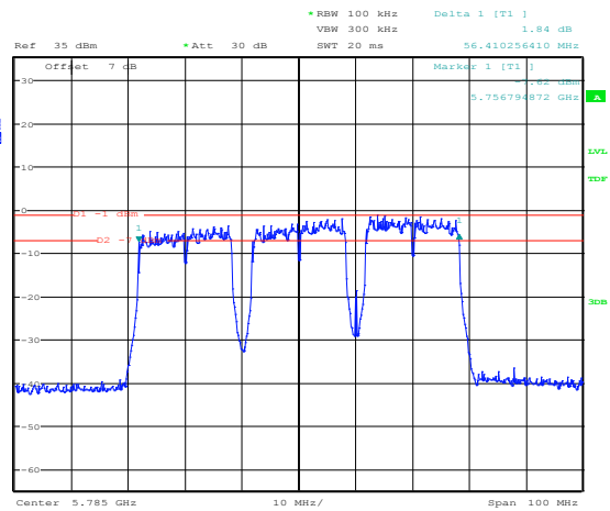
Figure 8.1-5: 6 dB bandwidth at top of the band, 2-carrier operation
