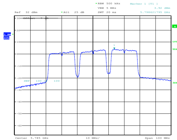
Figure 8.3-22: Conducted PPSD at the top of the band, 2-carrier operation, Canada
