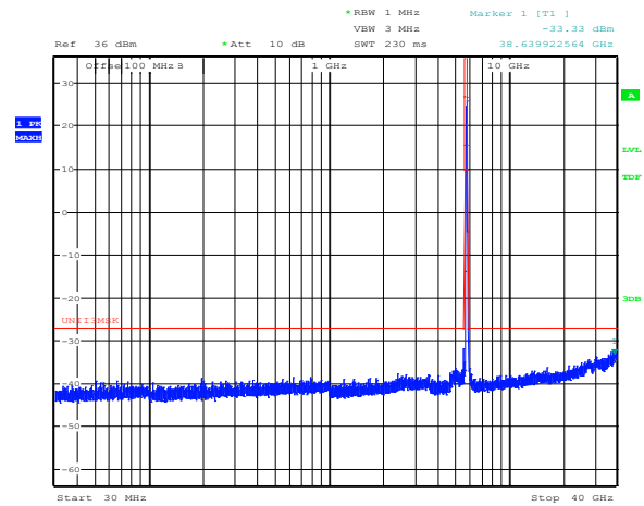
Figure 8.4-5: Peak conducted spurious emissions outside restricted bands at the top of the band, 2-carrier operation
