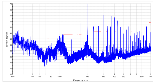
Radiated spurious emissions FCC 15.205 and RSS-Gen Restricted bands limits Peak max-hold
