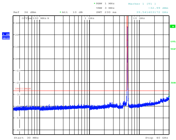
Figure 8.4-4: Peak conducted spurious emissions outside restricted bands at the bottom of the band, 2-carrier operation
