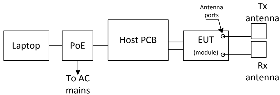
Figure 3.6-1: Setup diagram
