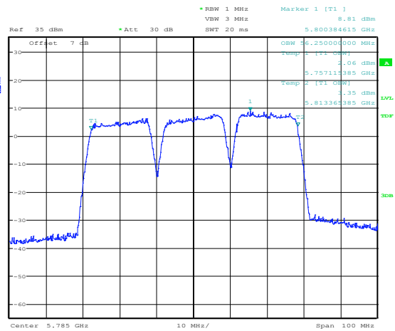
Figure 8.2-5: 99 % bandwidth at top of the band, 2-carrier operation
