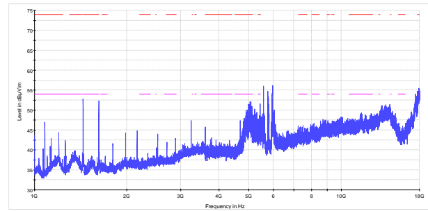
Legend: Radiated spurious emissions PK e , MAXH FCC 15.205 and RSS-Gen Restricted bands limits FCC 15.209 and RSS-210 limitline RB pk
