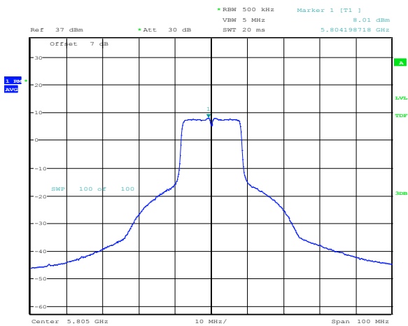
Figure 8.3-13: Conducted PPSD at mid channel, 1-carrier operation, 14 dBi antenna
