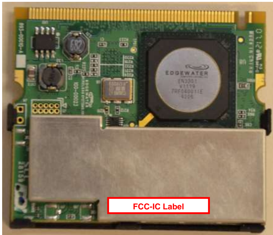
Figure 1 EWC24GWFR1 Radio Card FCC-IC Label Location
