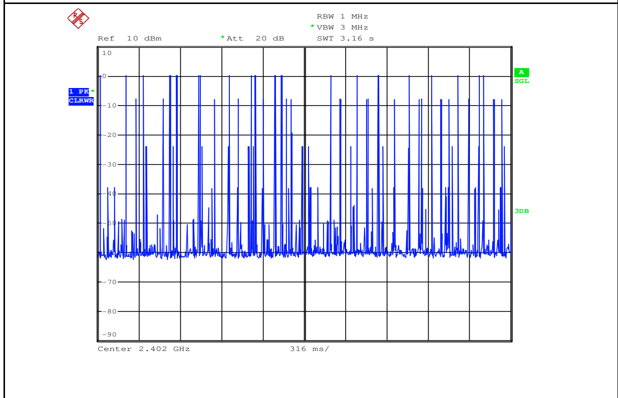
Dwell Time_DH5_2402
