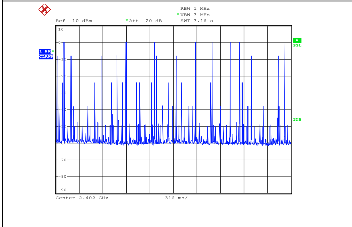
Dwell Time_2DH1_2402
