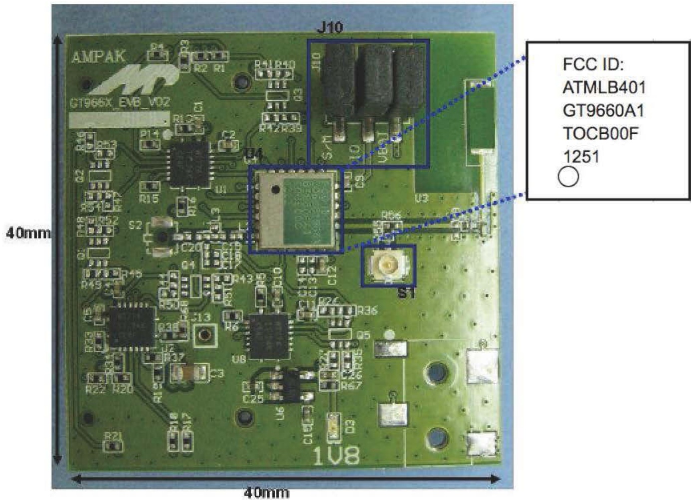
Figure1. Top view of GT966X EVB
