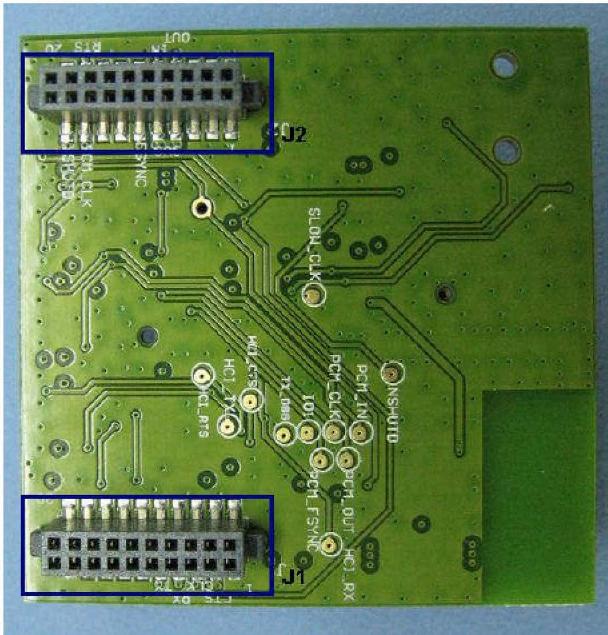
Figure2. Bottom view of GT966X EVB
