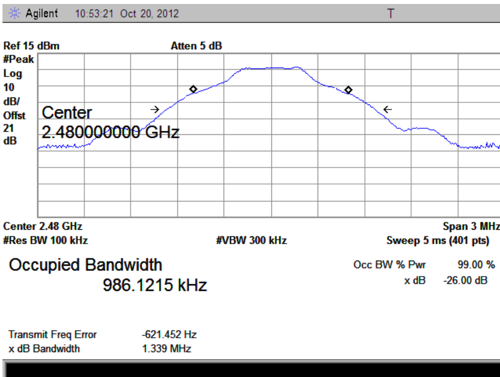
(Plot C1:Channel = 2480)
