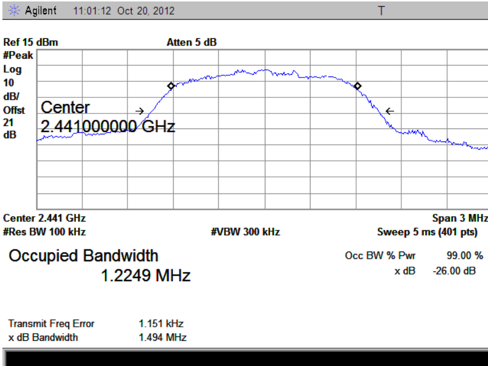
(Plot H1:Channel = 2441)
