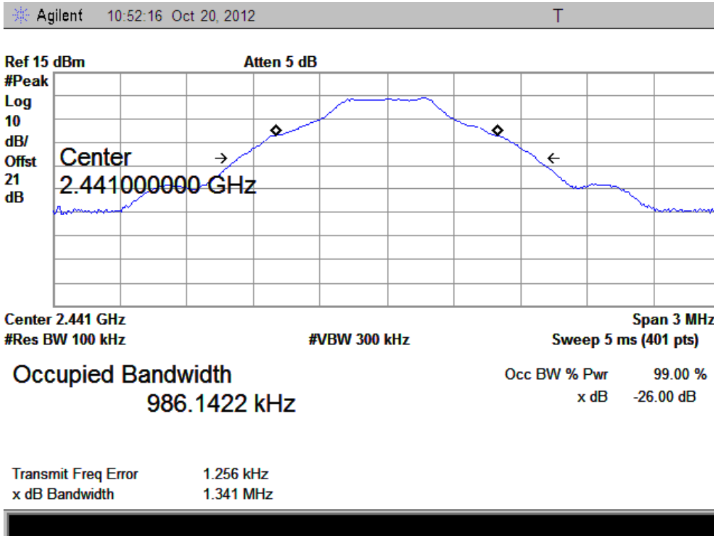
(Plot B1:Channel = 2441)
