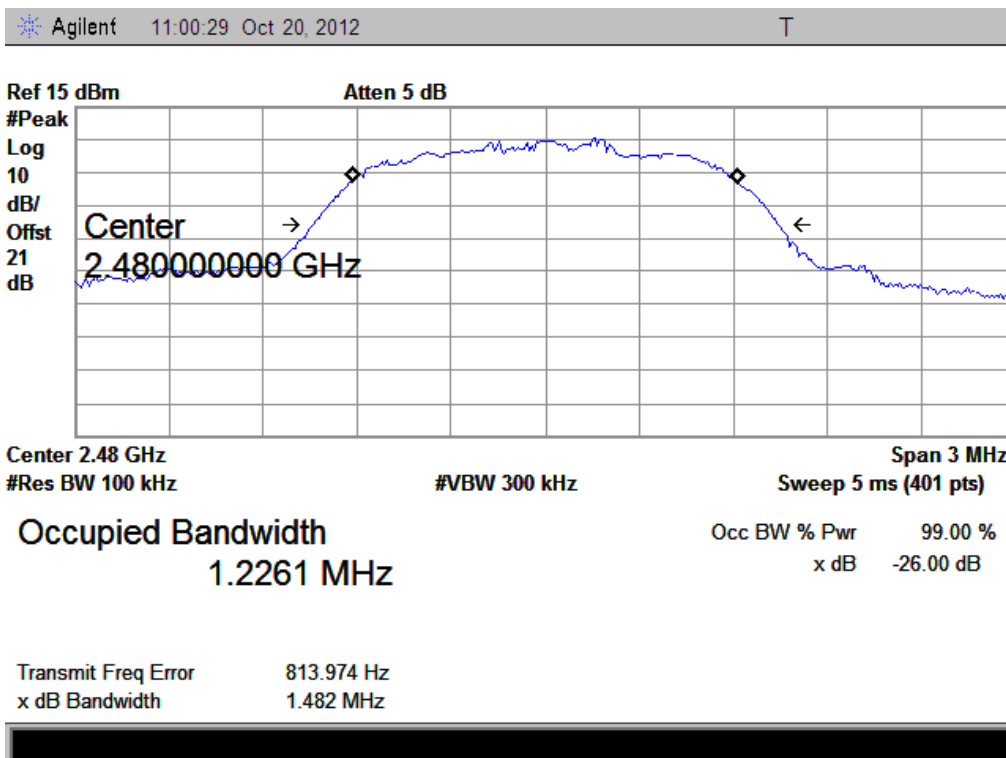
(Plot I1:Channel = 2480)
