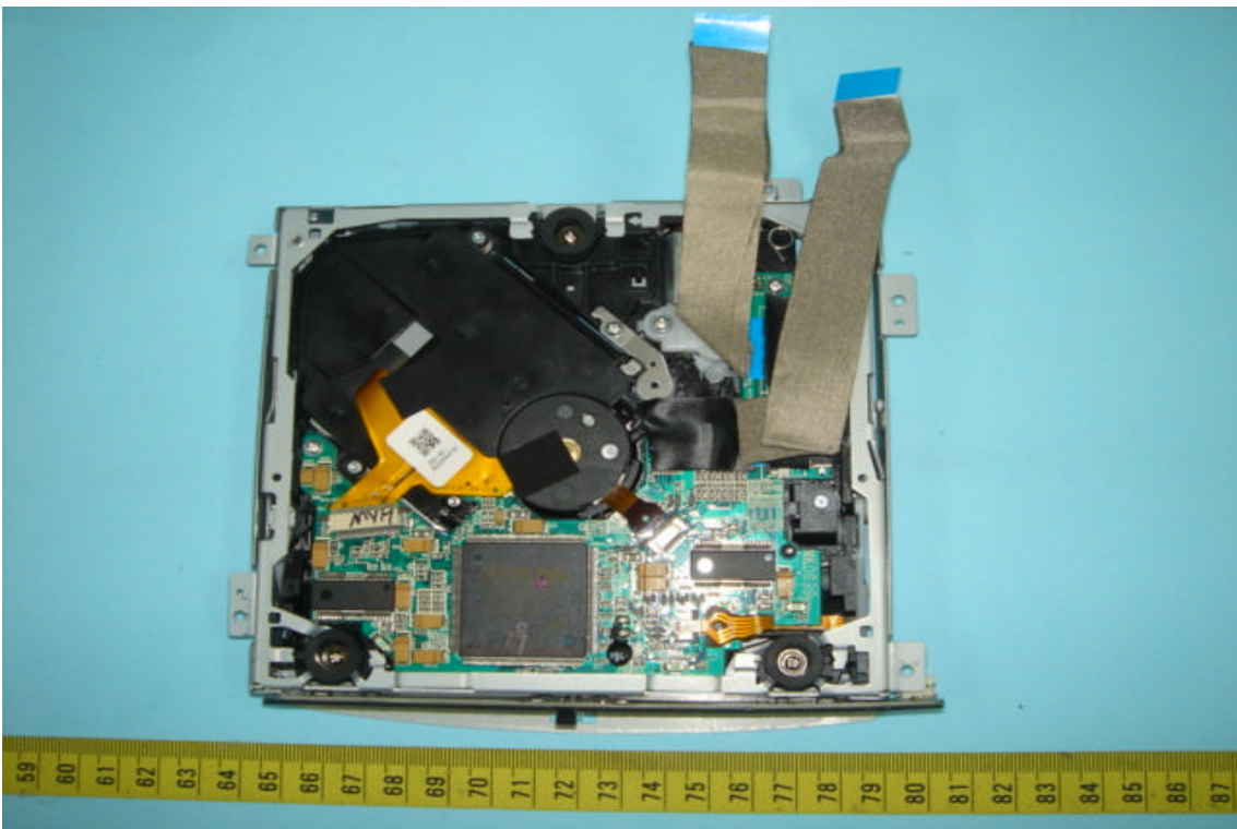
11. Internal View of EUT
