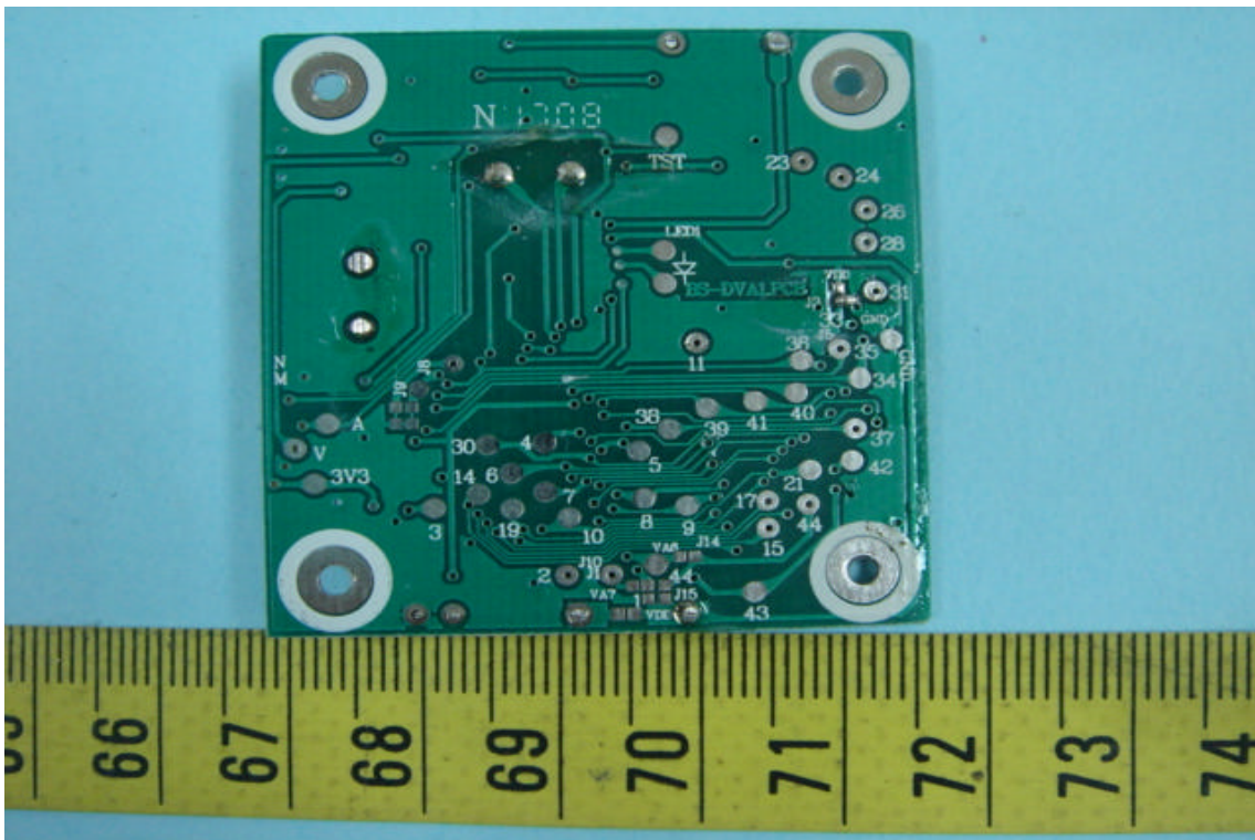
20. Solder View of PCB
