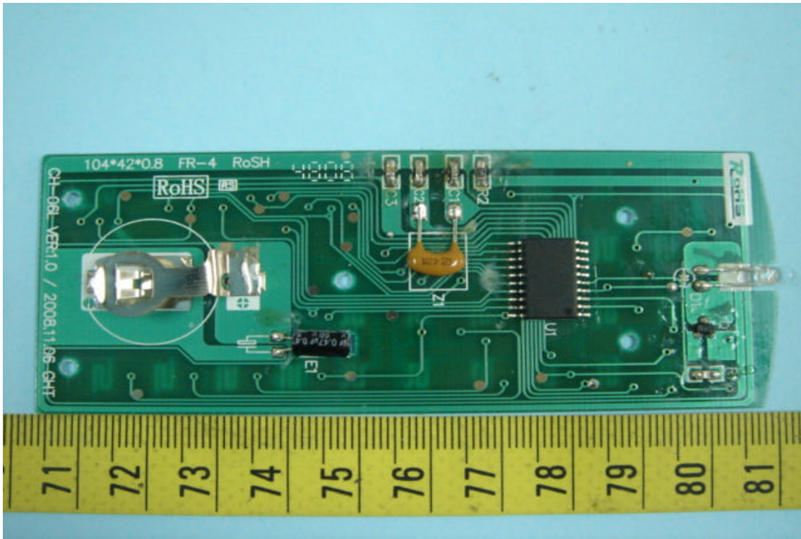
27. Component View of Remote Controller
