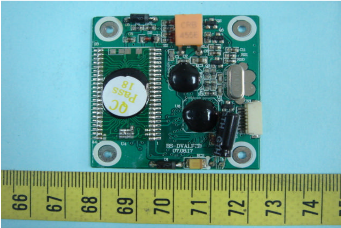
19. Component View of PCB
