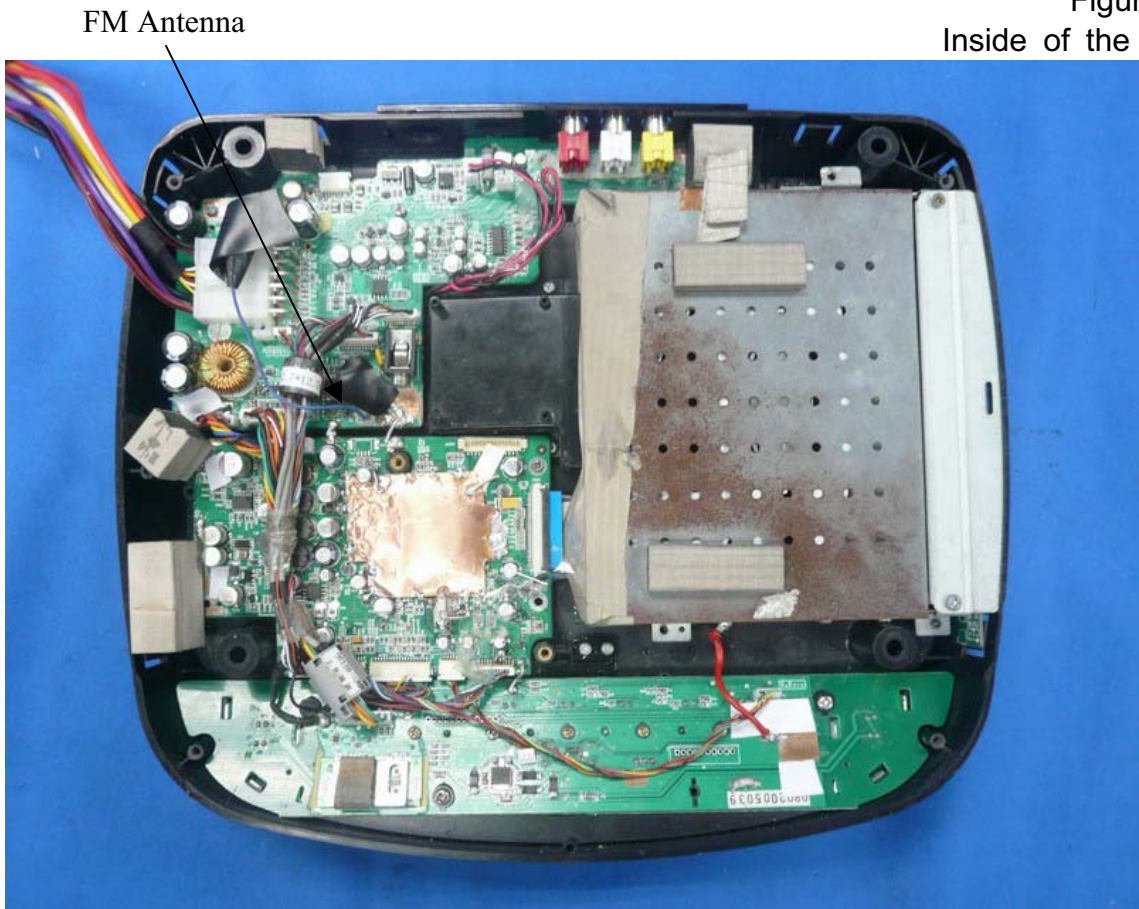
Figure 6 Inside of the EUT
