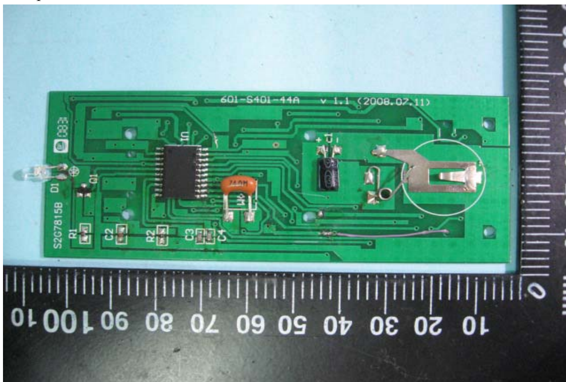
Component View of Remote Controller's PCB
