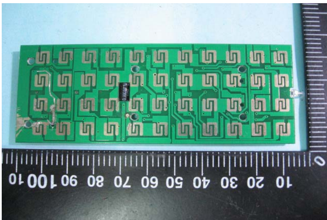
Solder View of Remote Controller's PCB
