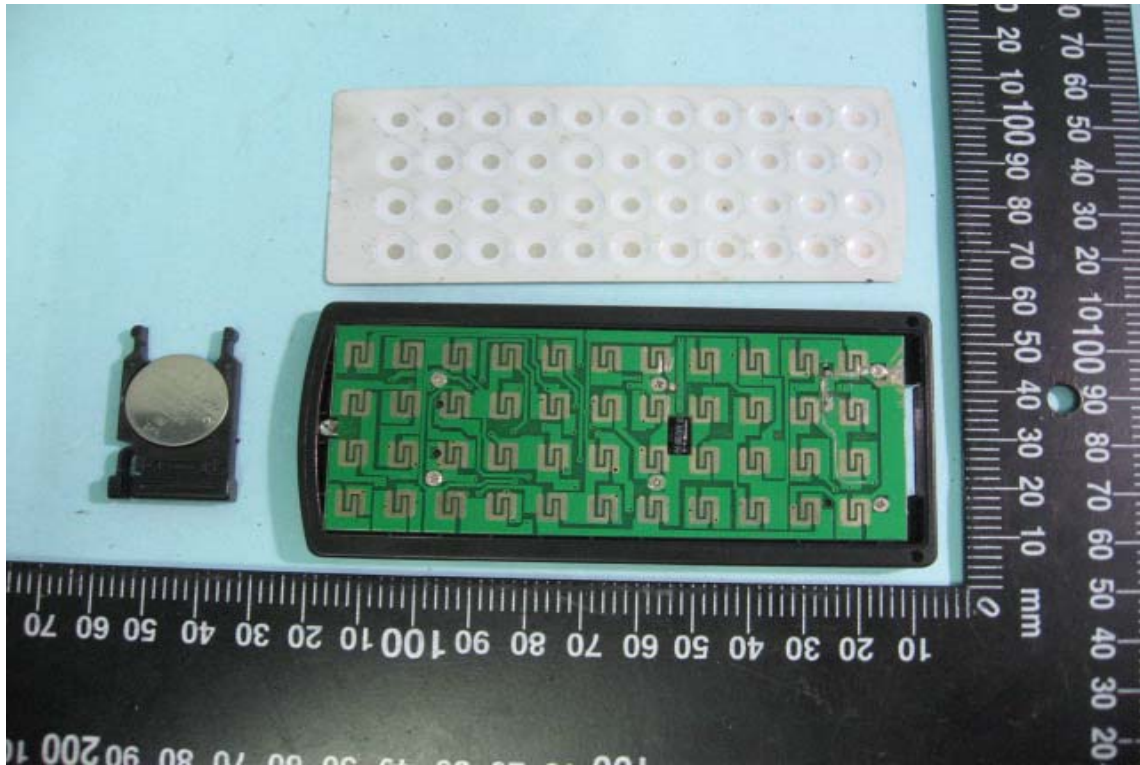
Internal View of Remote Controller
