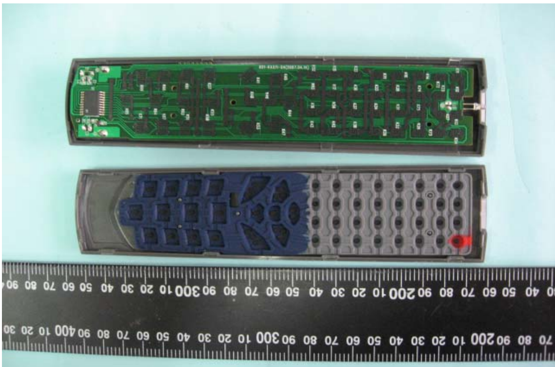
25. Internal View of Remote Controller
