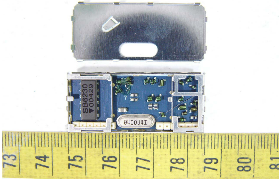
32. Component View of PCB
