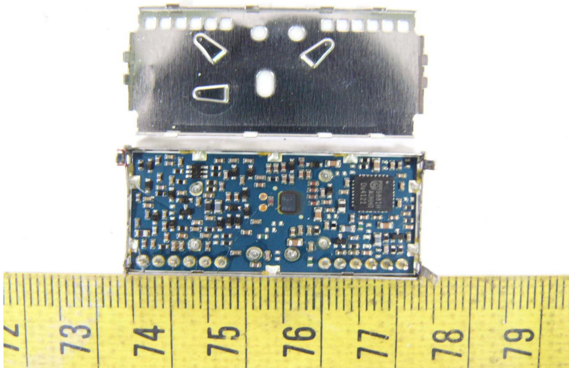
33. Solder View of PCB
