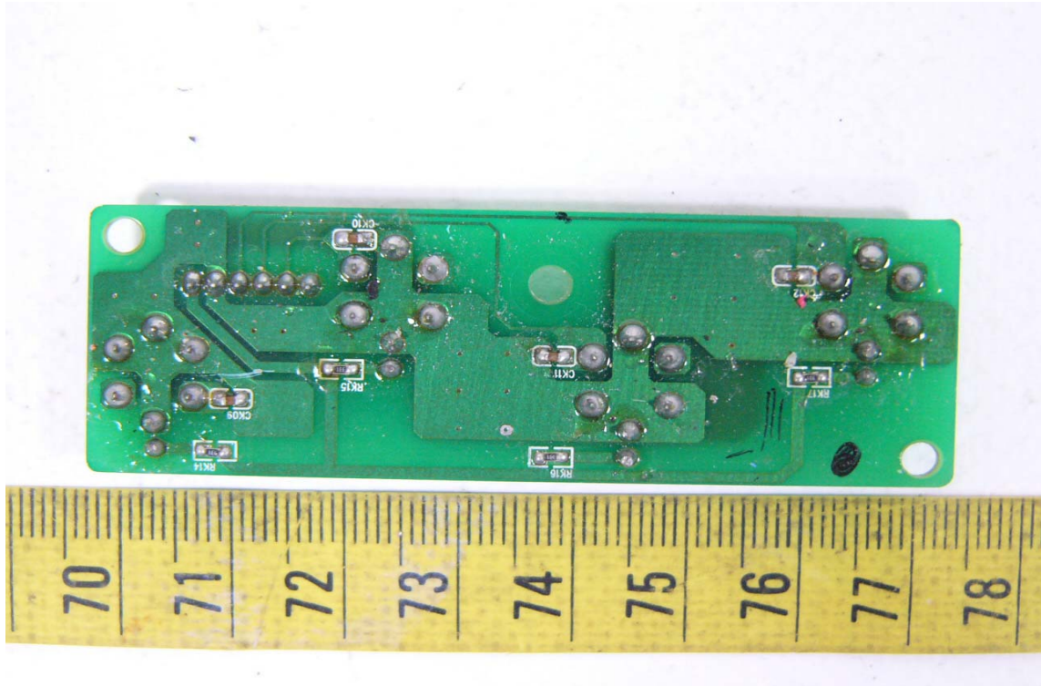
24. Solder View of PCB
