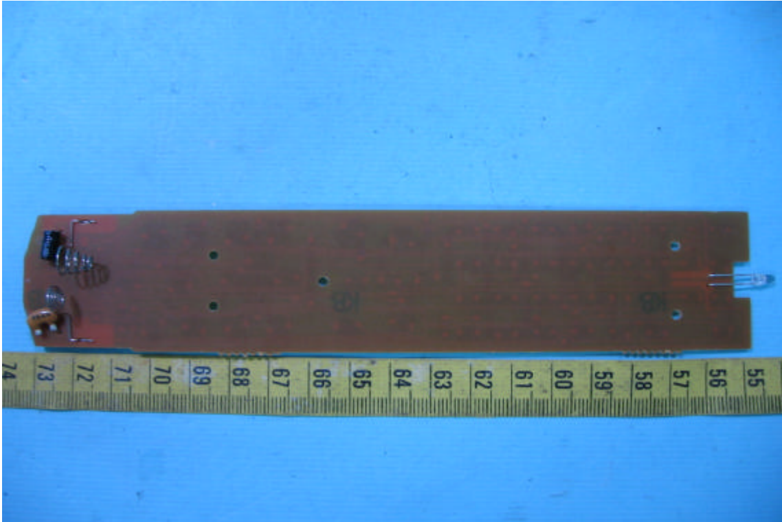
Component View of the Remote Control's Main PCB
