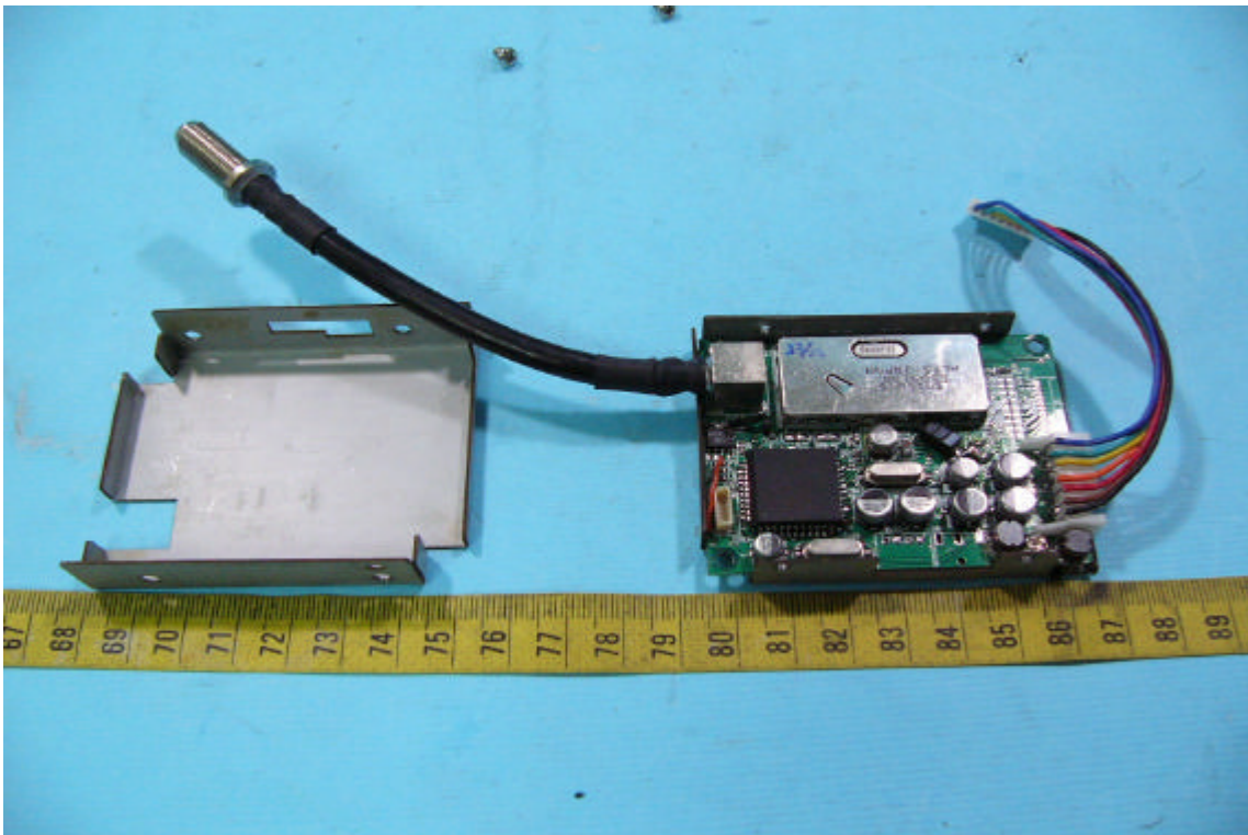
Internal View of the TV Tuner
