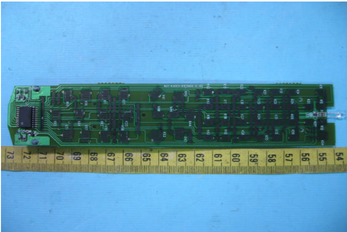
Solder View of the Remote Control's Main PCB
