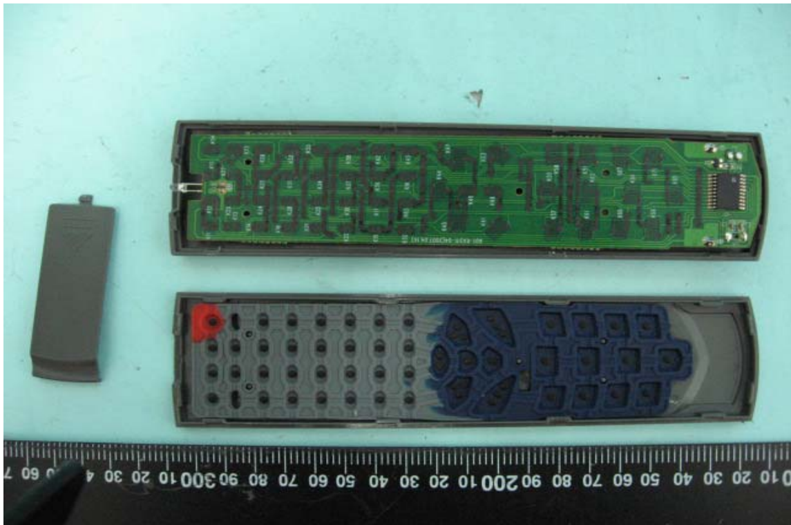
Internal View of Remote Controller's PCB
