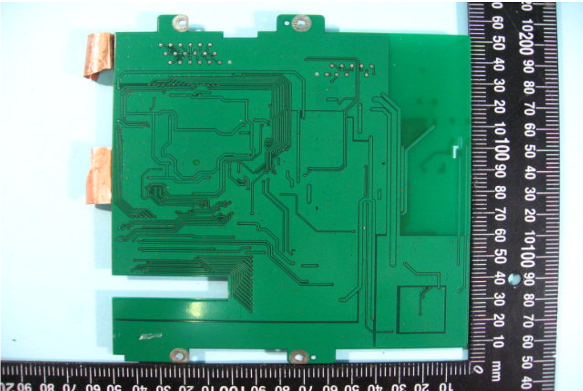
21. Solder View of PCB
