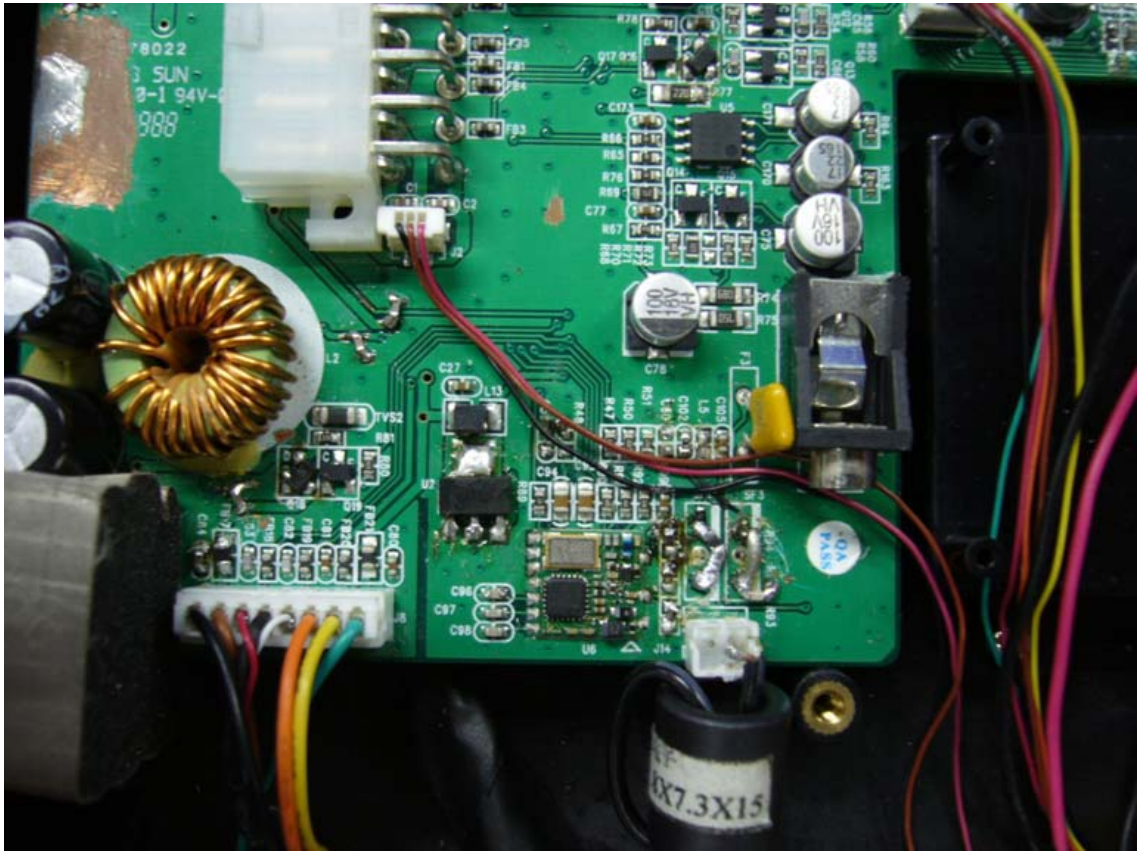
Figure 31 RF Module of the EUT
