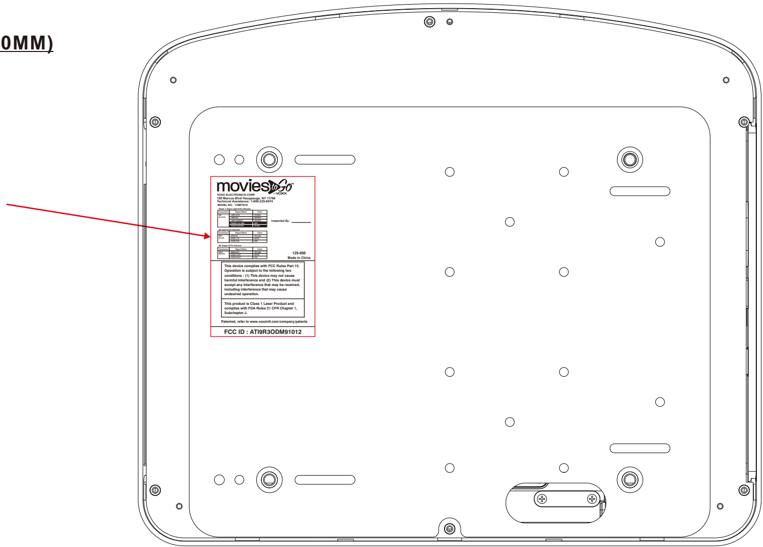
UNIT BACK VIEW
