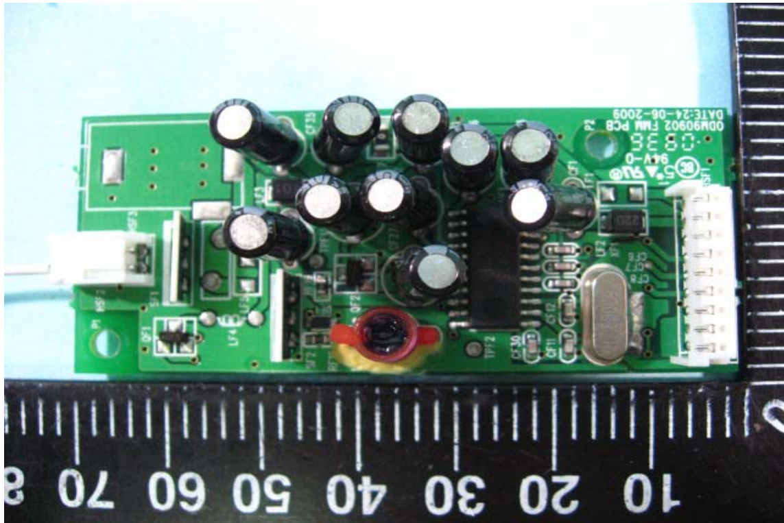
Component View of FM transmitter PCB
