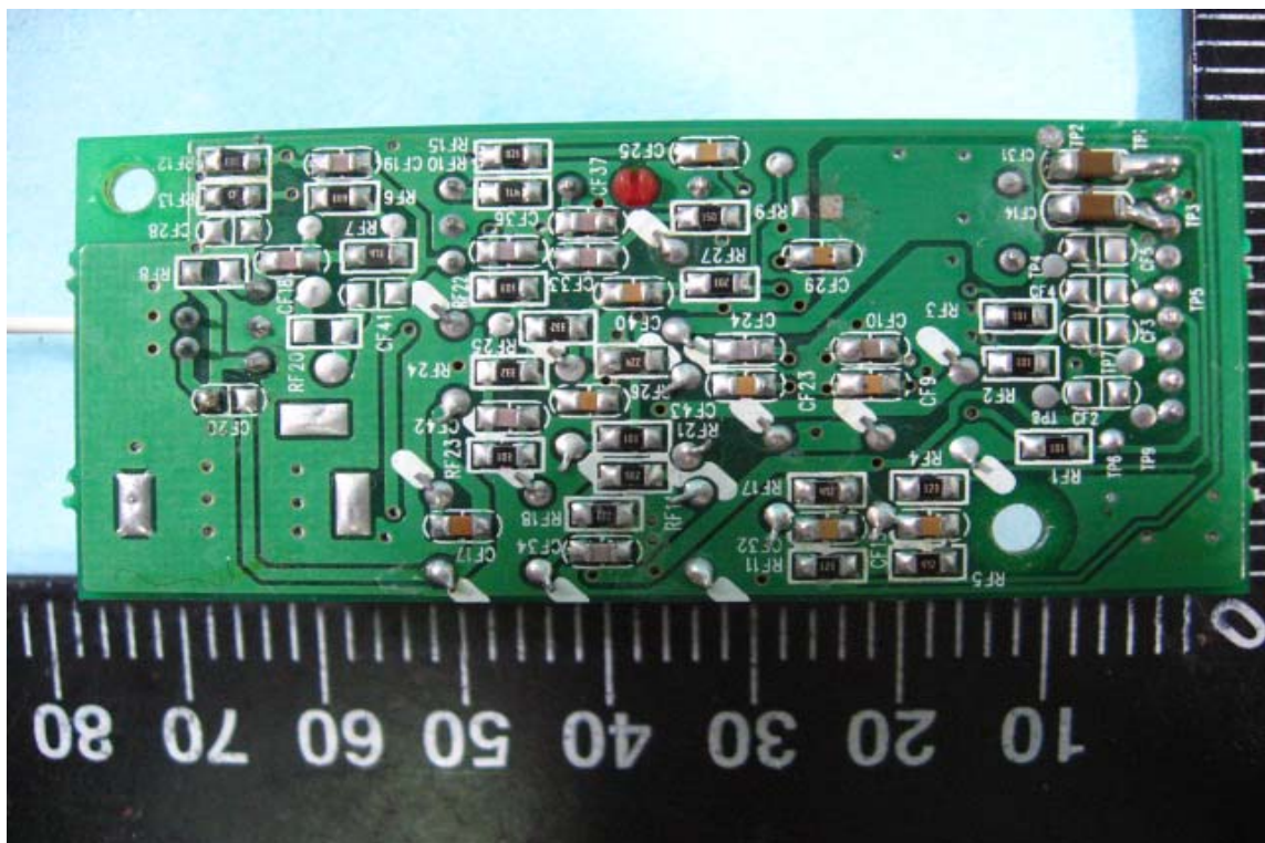
Solder View of FM transmitter PCB
