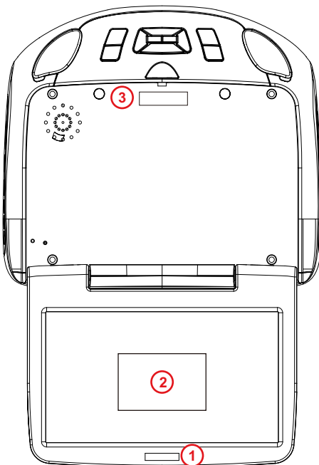
1. LOGO PLATE (32 x 6.5MM) (50-NH-20010G)
