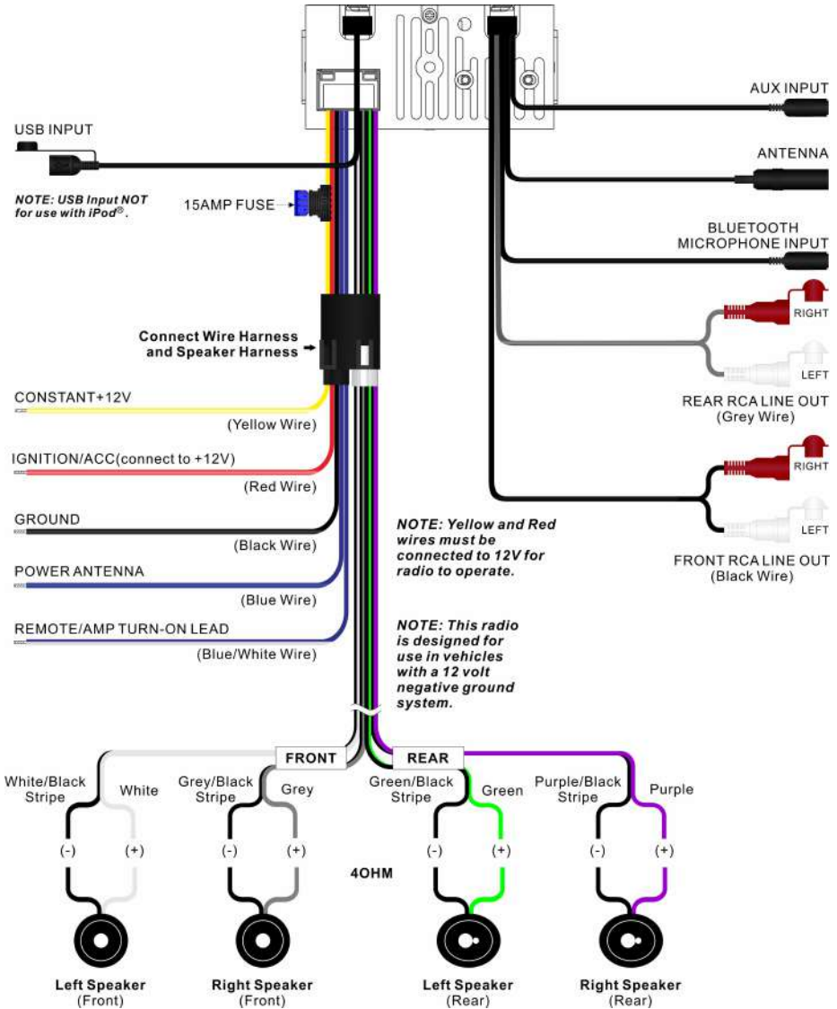
Figure 5 - Wiring Diagram
