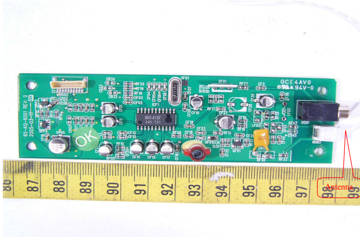
20. Component View of PCB
