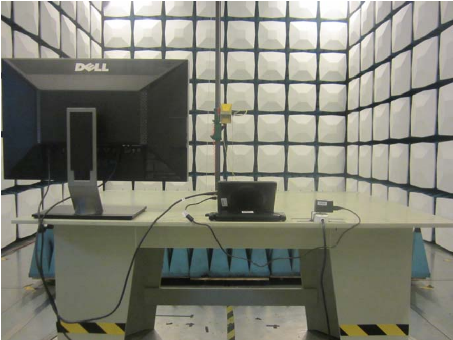
Radiated Emission Above 1GHz - Rear View (HDMI Playing) (AC mains input)
