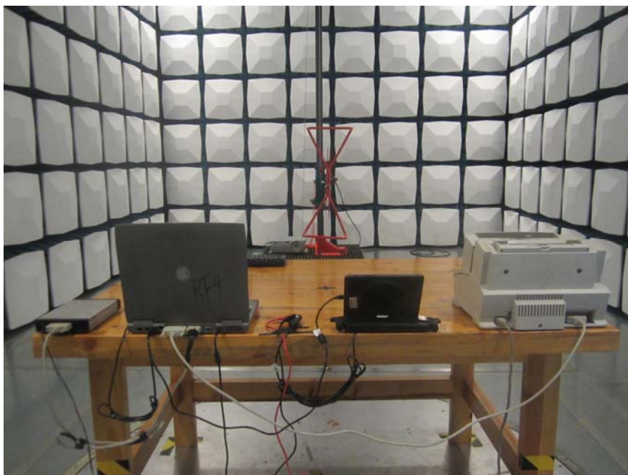
Radiated Emission Below 1GHz - Rear View (USB Downloading) (DC input)
