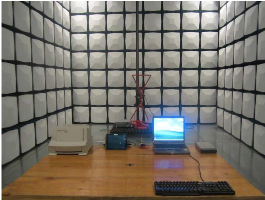
Radiated Emission Below 1GHz -Front View (USB Downloading) (DC input)
