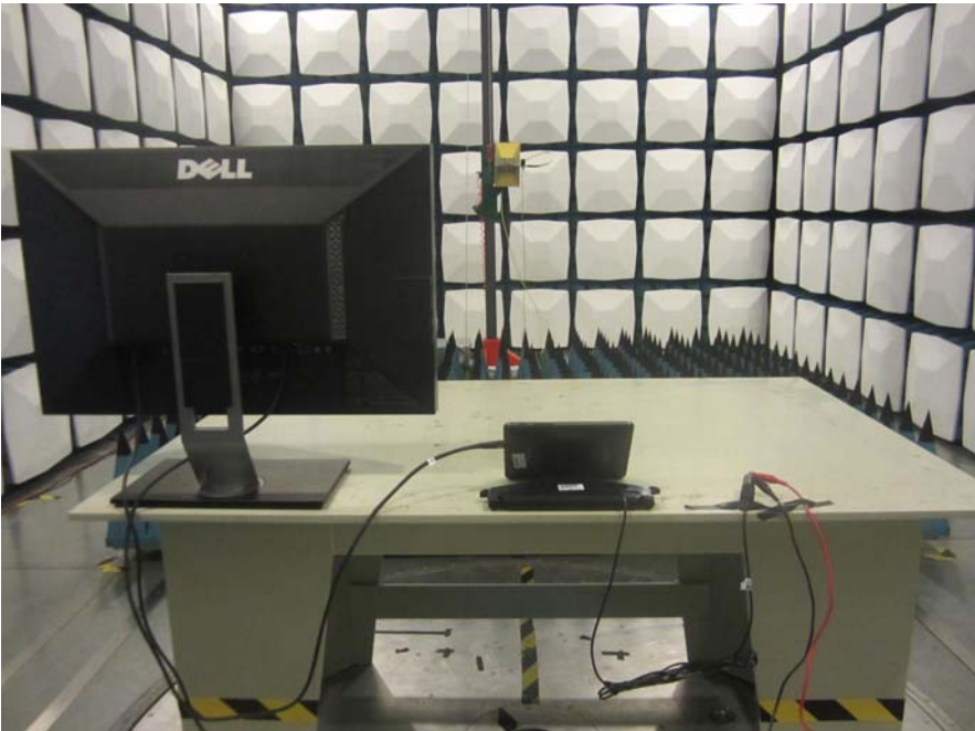
Radiated Emission Above 1GHz - Rear View (HDMI Playing) DC input)
