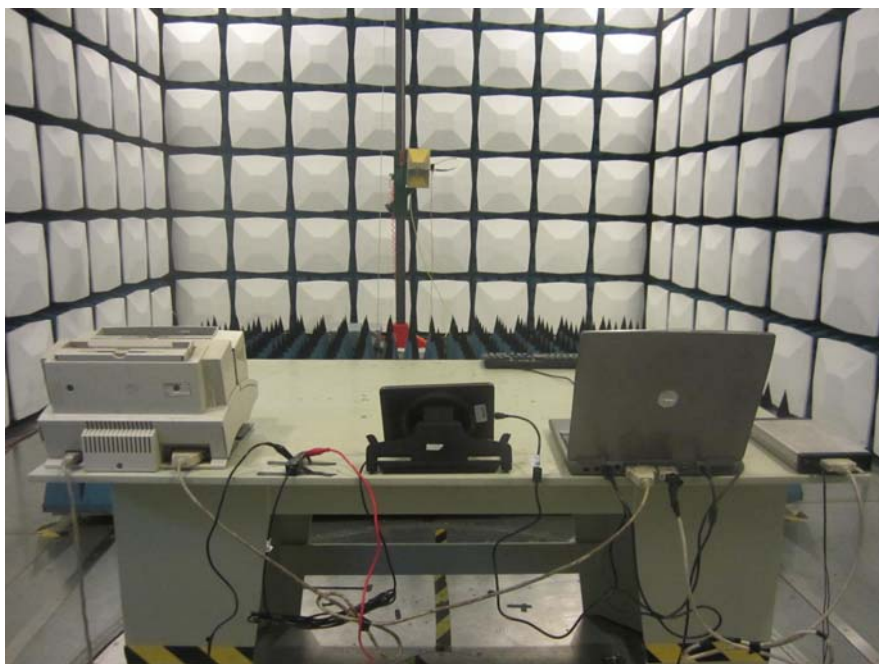
Radiated Emission Above 1GHz - Rear View (USB Downloading) (DC input)
