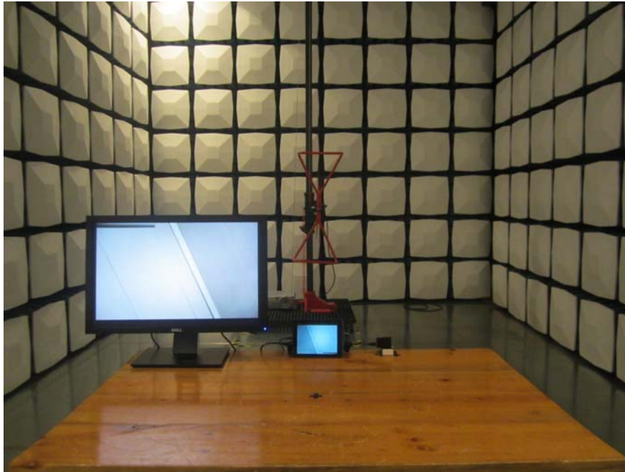
Radiated Emission Below 1GHz - Rear View (HDMI Playing) (AC mains input)
