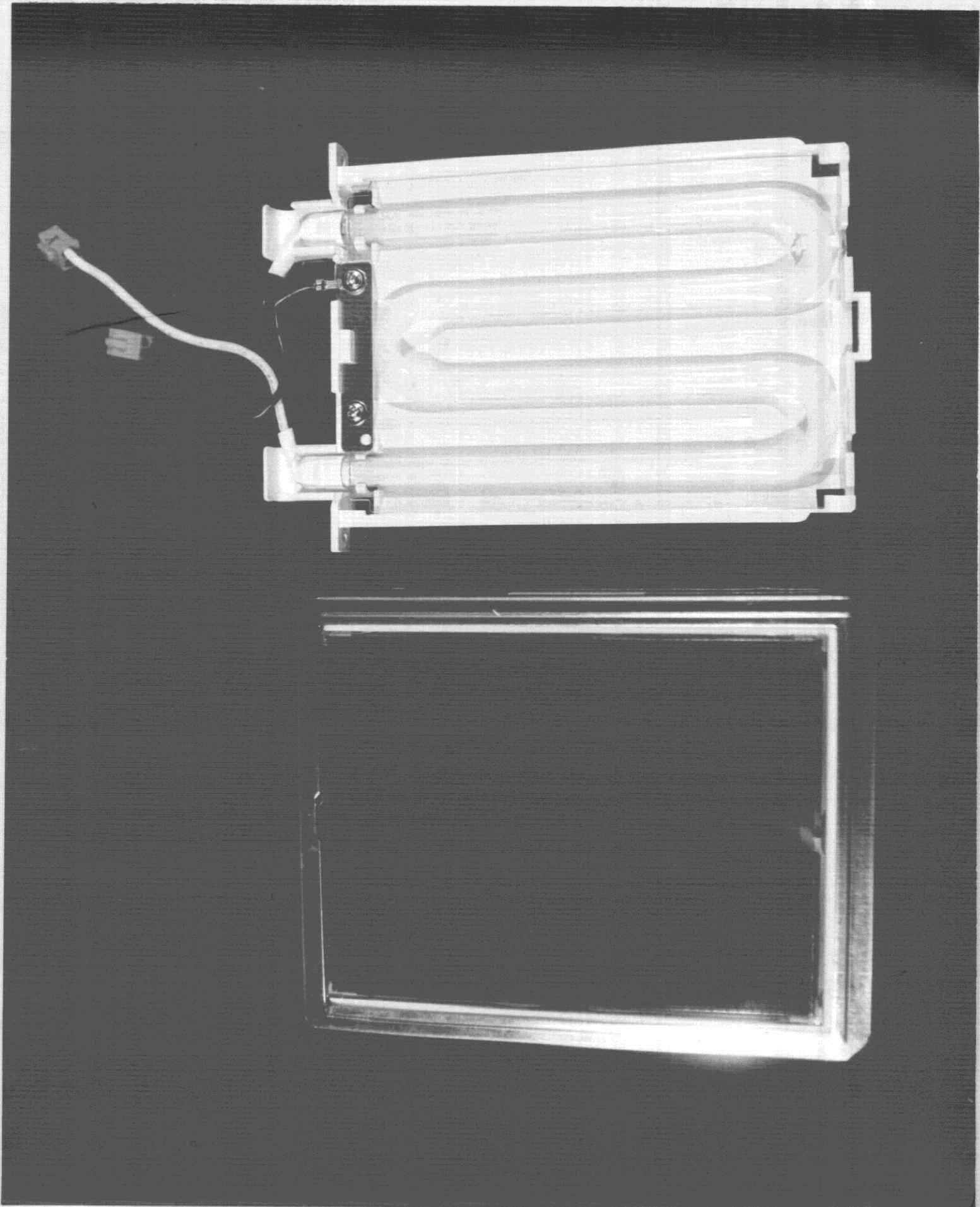
Front View of LCD Panel Module
