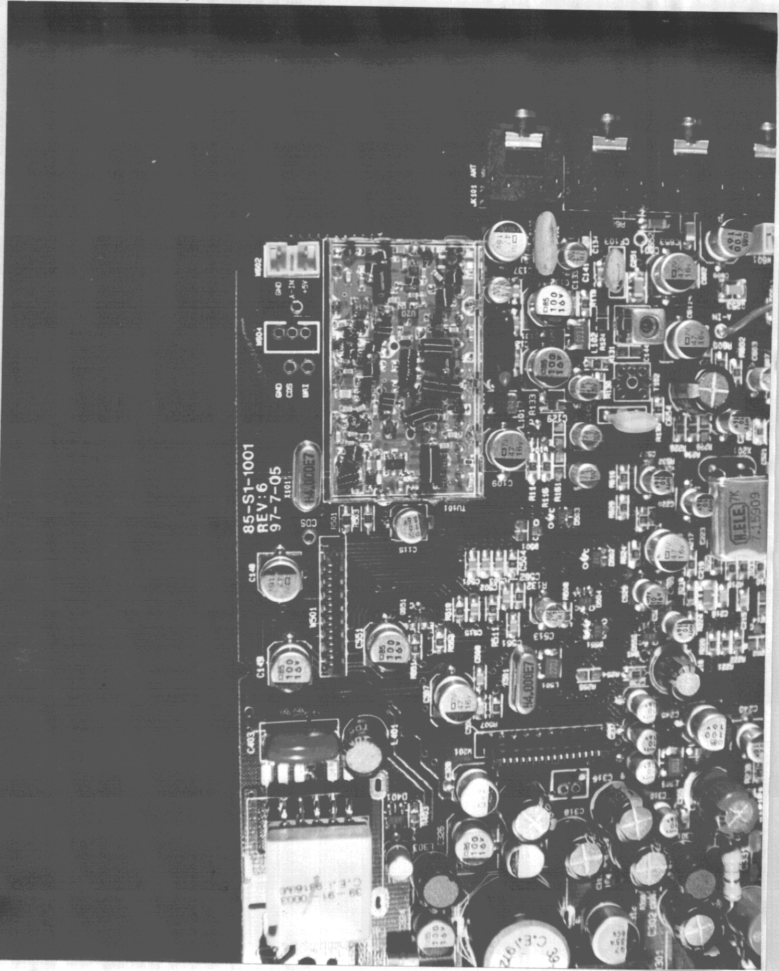
Component View 2 of Main Board
