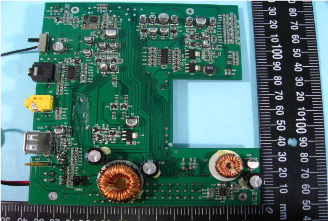
12. Component View of PCB
