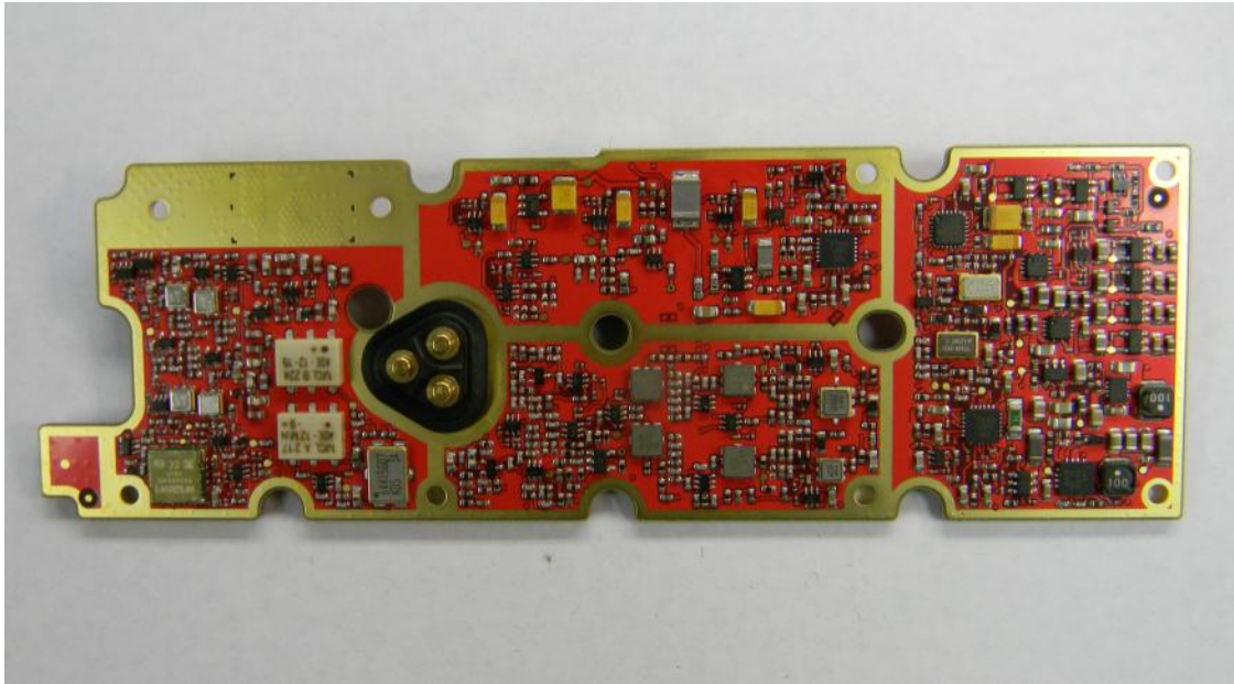
RF PC Board Back
