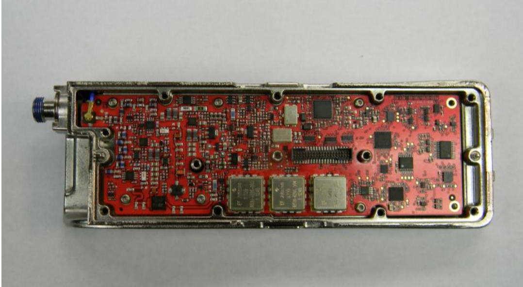
Radio Chassis Assembly with Inner Shield Removed Showing RF PC Board
