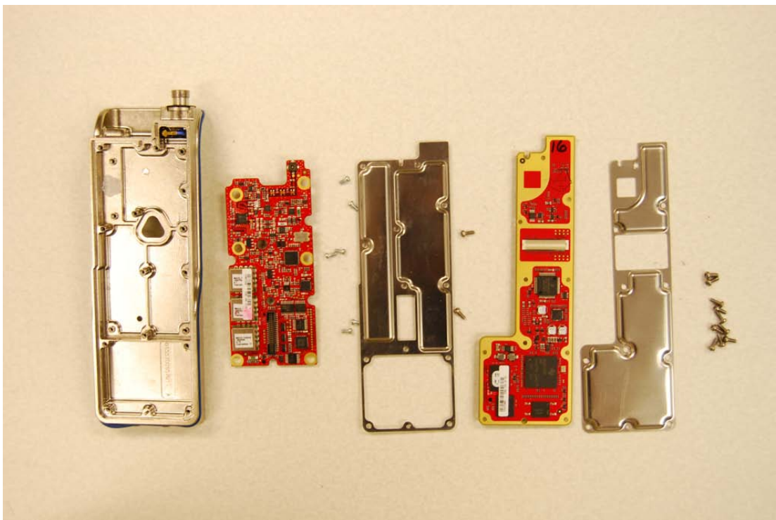
Radio Chassis Assembly Breakout
