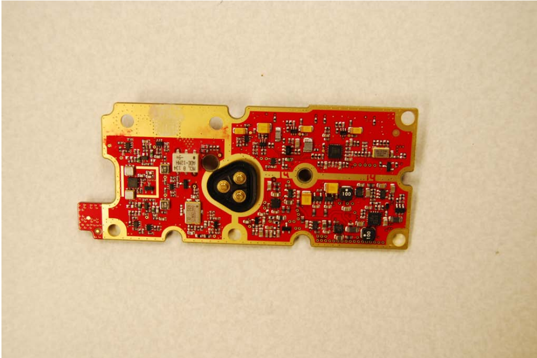
RF PC Board Back
