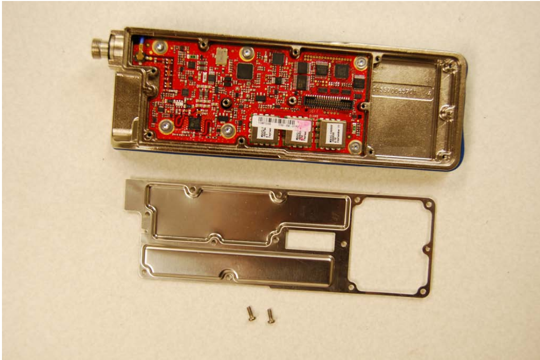
Radio Chassis Assembly with Inner Shield Removed Showing RF PC Board
