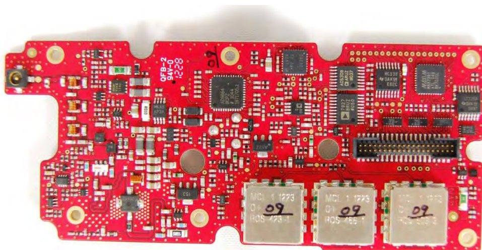
Radio Chassis Assembly with Inner Shield Removed Showing RF PC Board
