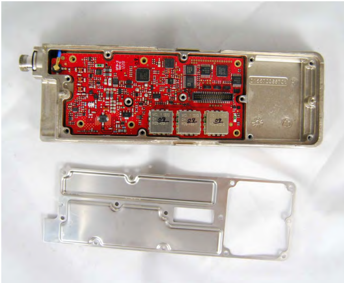
Radio Chassis Assembly with Inner Shield Removed Showing RF PC Board
