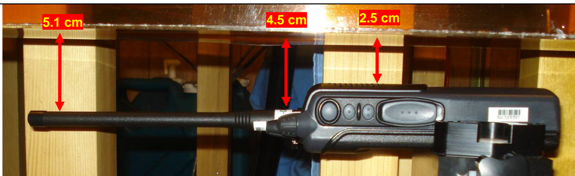
Face-held test setup – Radio with Antenna 1, Battery a
