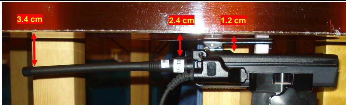
Body-worn Test Setup – Radio with Antenna 1, Body-worn acc. 1, Battery a, Audio acc. 1
