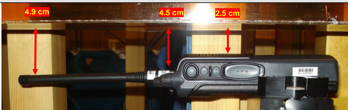
Face-held test setup - Radio with Antenna 2, Battery a
