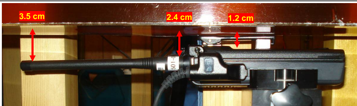
Body-worn Test Setup - Radio with Antenna 2, Body-worn acc. 1, Battery a, Audio acc. 1
