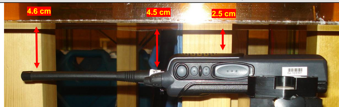
Face-held test setup - Radio with Antenna 3, Battery a
