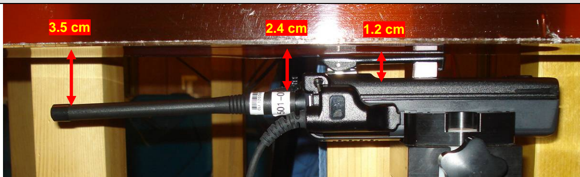
Body-worn Test Setup - Radio with Antenna 3, Body-worn acc. 1, Battery a, Audio acc. 1
